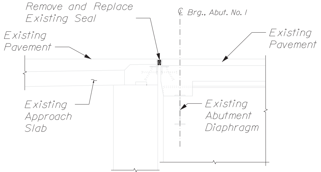
ABUTMENT NO. 1 (EXISTING)
