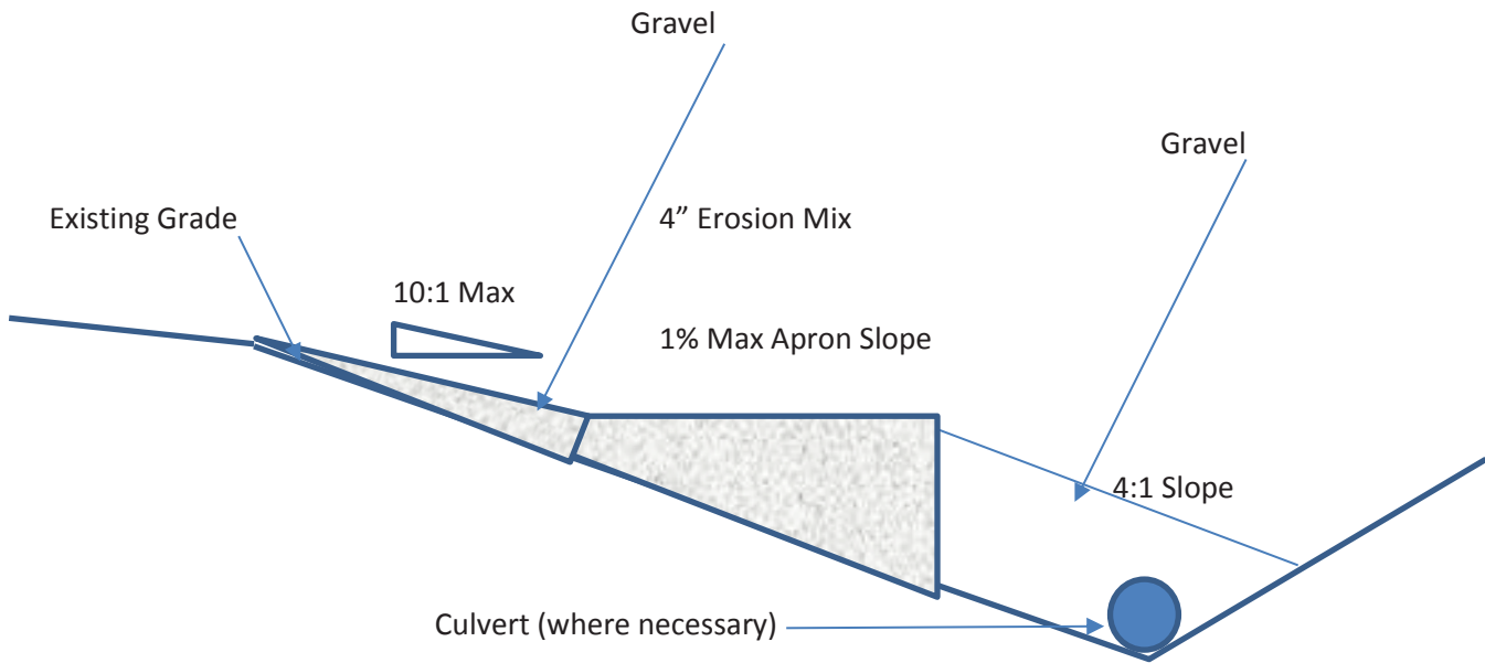
TYPICAL GRAVEL PAD SECTION Not to scale
