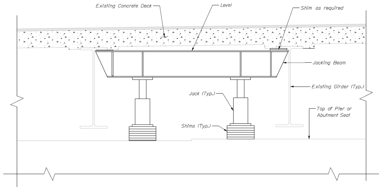
CONCEPTUAL JACKING DETAIL
