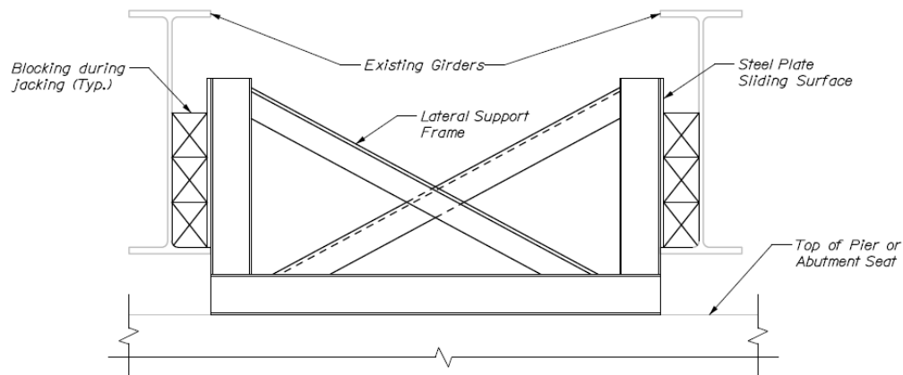
CONCEPTUAL LATERAL SUPPORT FRAME
