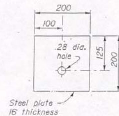
BEARING PLATE
