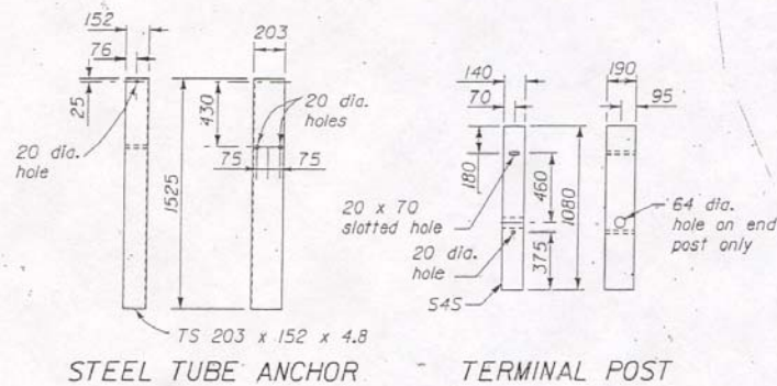
ELEVATION TYPE I END SECTION ASSEMBLY
