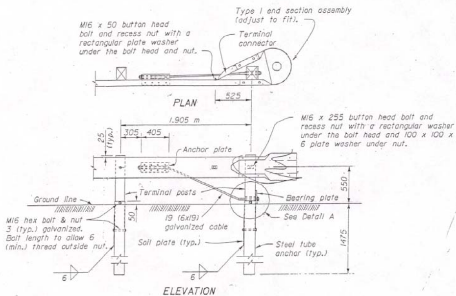
ANCHORAGE ASSEMBLY
