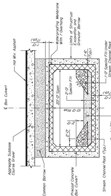
BOX CULVERT SECTION
