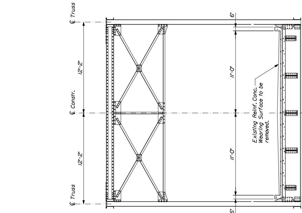
EXISTING BRIDGE SECTION
