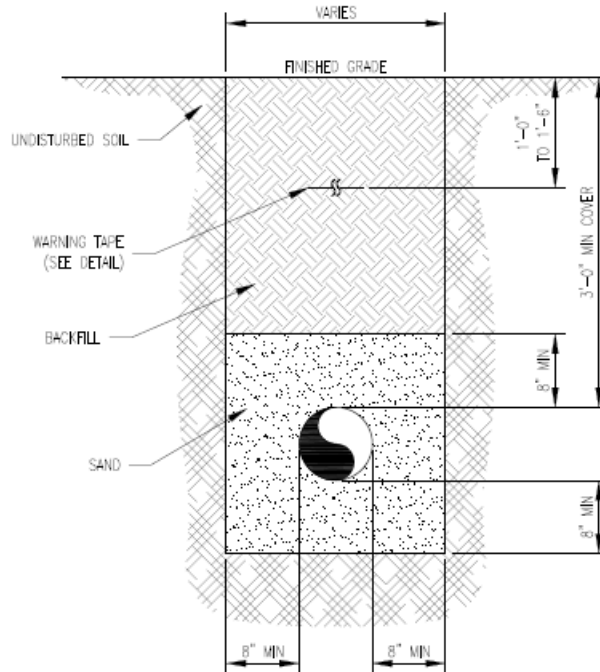
TYPICAL TRENCH DETAIL SCALE: 1" = 1'-0"
