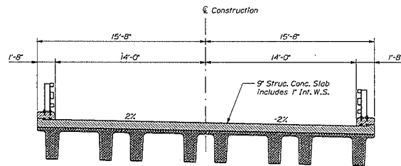
PROPOSED TRANSVERSE SECTION NEXT 36 F Beams
