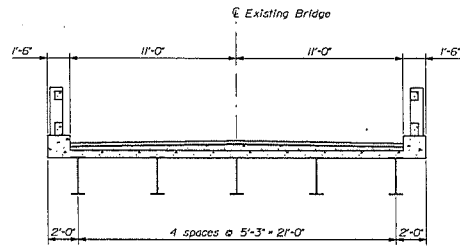
EXISTING TRANSVERSE SECTION
