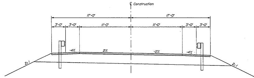
PROPOSED APPROACH GUARDRAIL SECTION 4" Hot Mix Asphalt 24" Aggregate Subbase Course - Gravel
