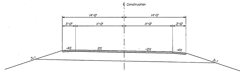
PROPOSED APPROACH SECTION 4" Hot Mix Asphalt 24" Aggregate Subbase Course - Gravel
