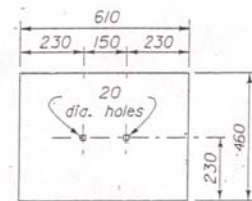
ANCHORAGE ASSEMBLY
