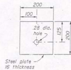
BEARING PLATE
