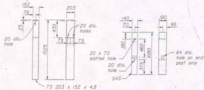
STEEL TUBE ANCHOR TERMINAL POST
