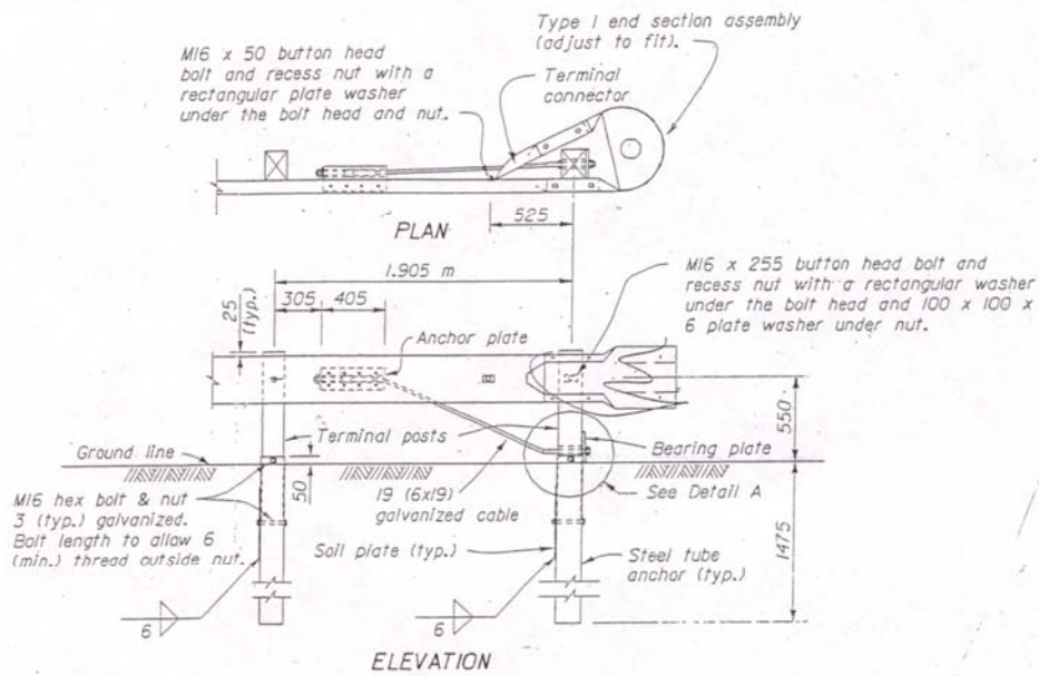
ANCHORAGE ASSEMBLY
