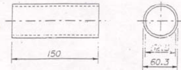
GALVANIZED STANDARD PIPE POST SLEEVE
