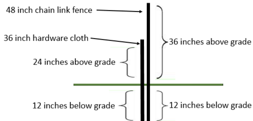
Figure 1, Side view of fence detail (not to scale)
