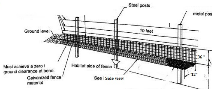
3a Apron fence schematic
