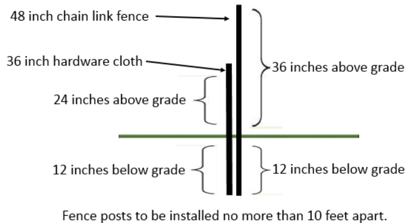
Figure 1, Side view of fence detail (not to scale)
