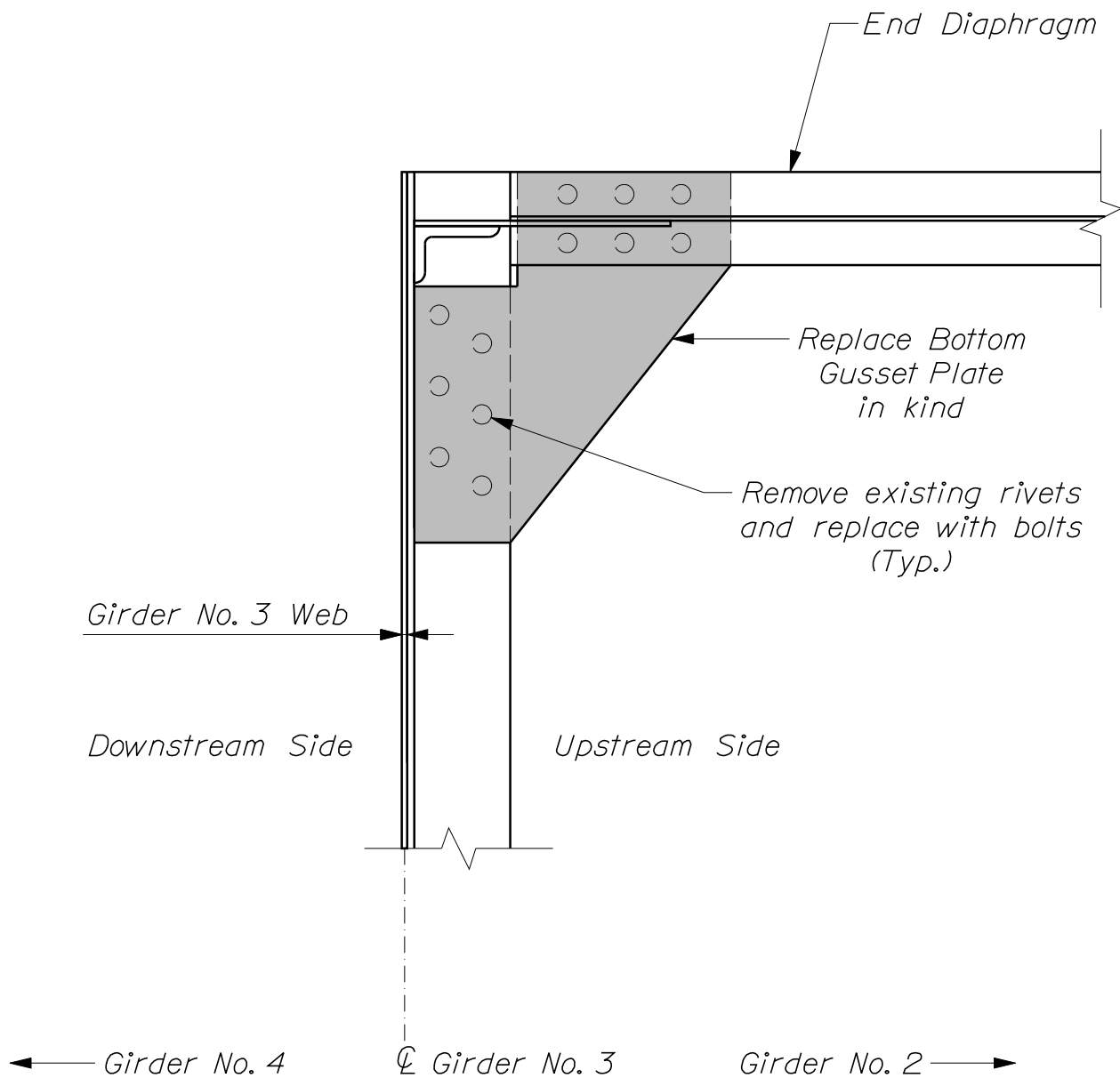
PLAN Bangor End River Span
