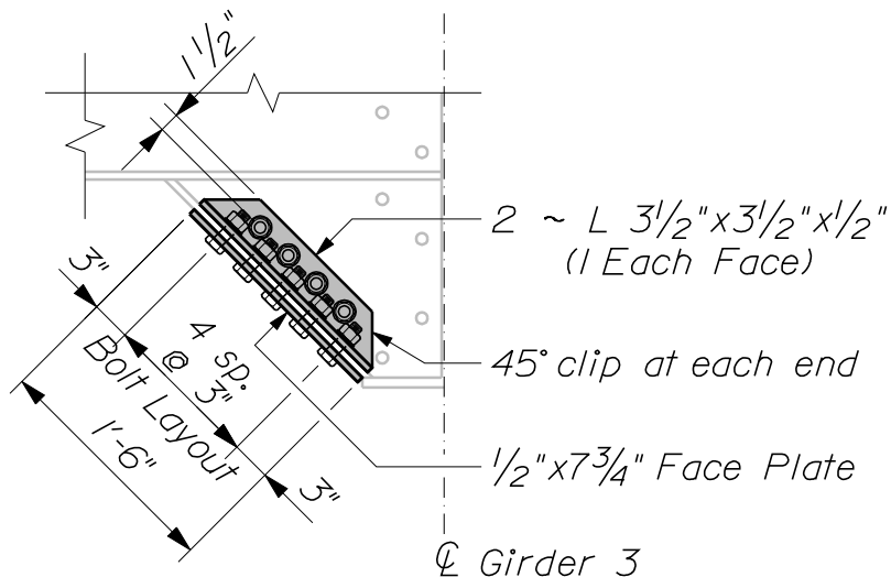
DETAIL
