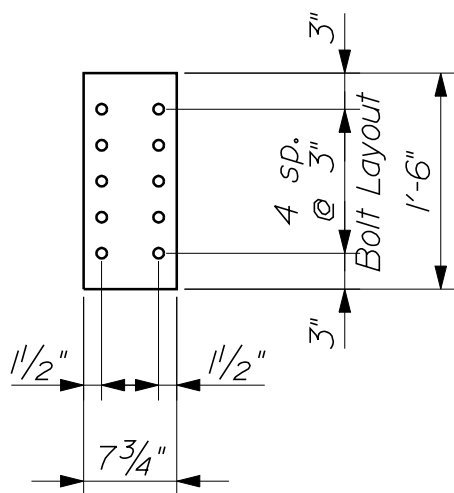
FACE PLATE
