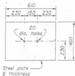
SOIL PLATE (2 reqd.)
