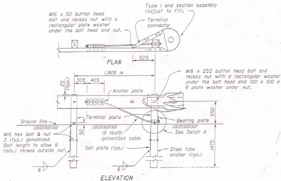
ANCHORAGE ASSEMBLY
