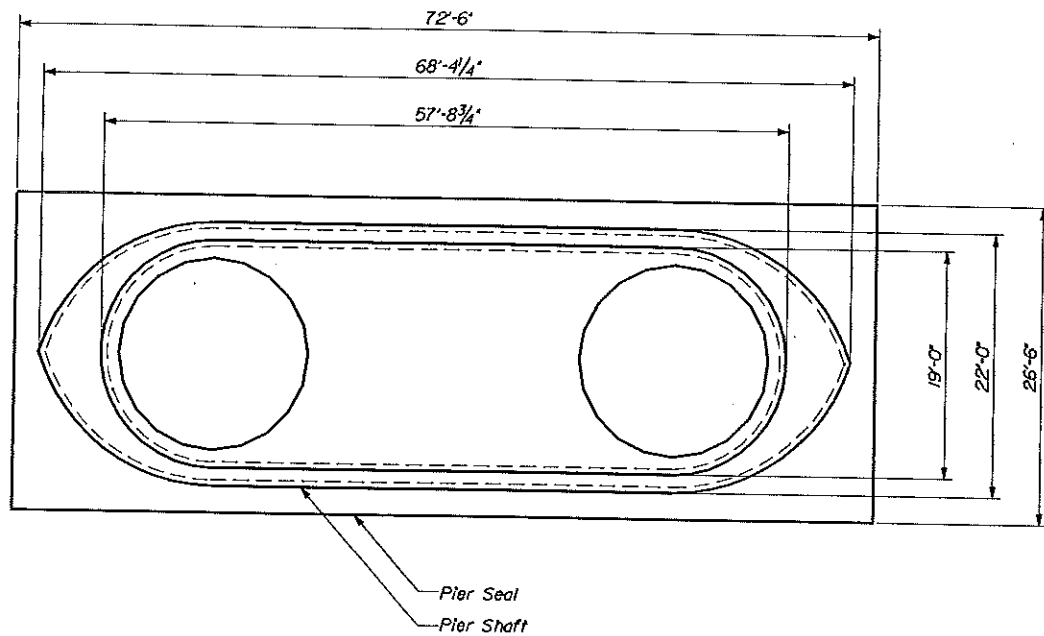
TYPICAL PIER PLAN Existing Piers to Remain
