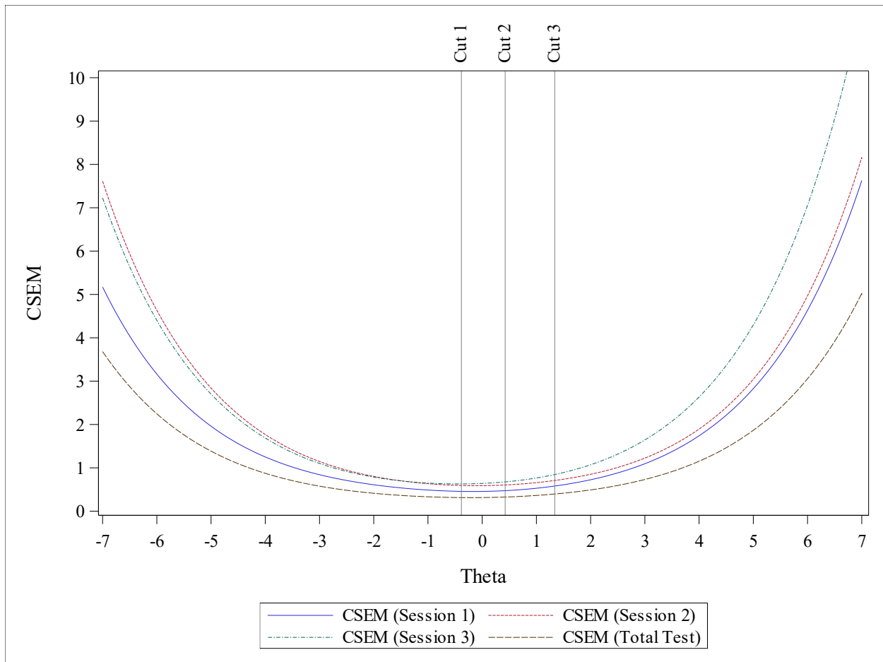
Figure 7. Grade 5 Conditional Standard Error of Measurement for 2025 Form
