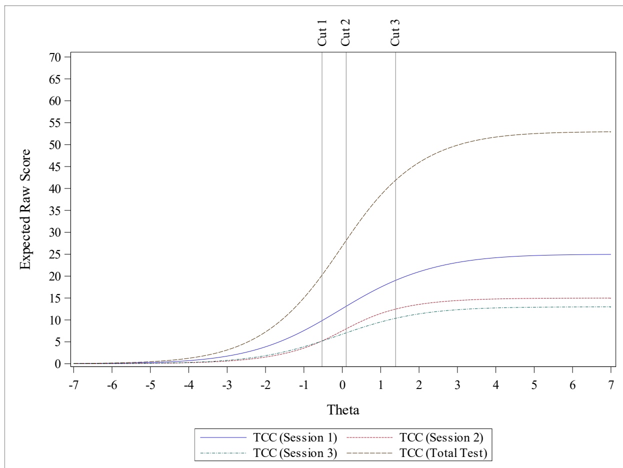
Figure 14. High School Test Characteristic Curve for 2025 Form
