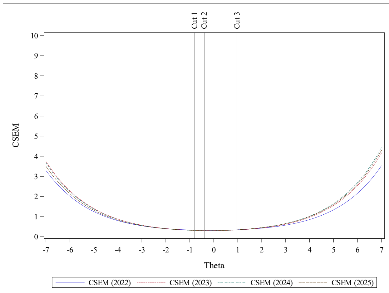
Figure 19. Grade 8 Conditional Standard Errors of Measurement 2022–2025
