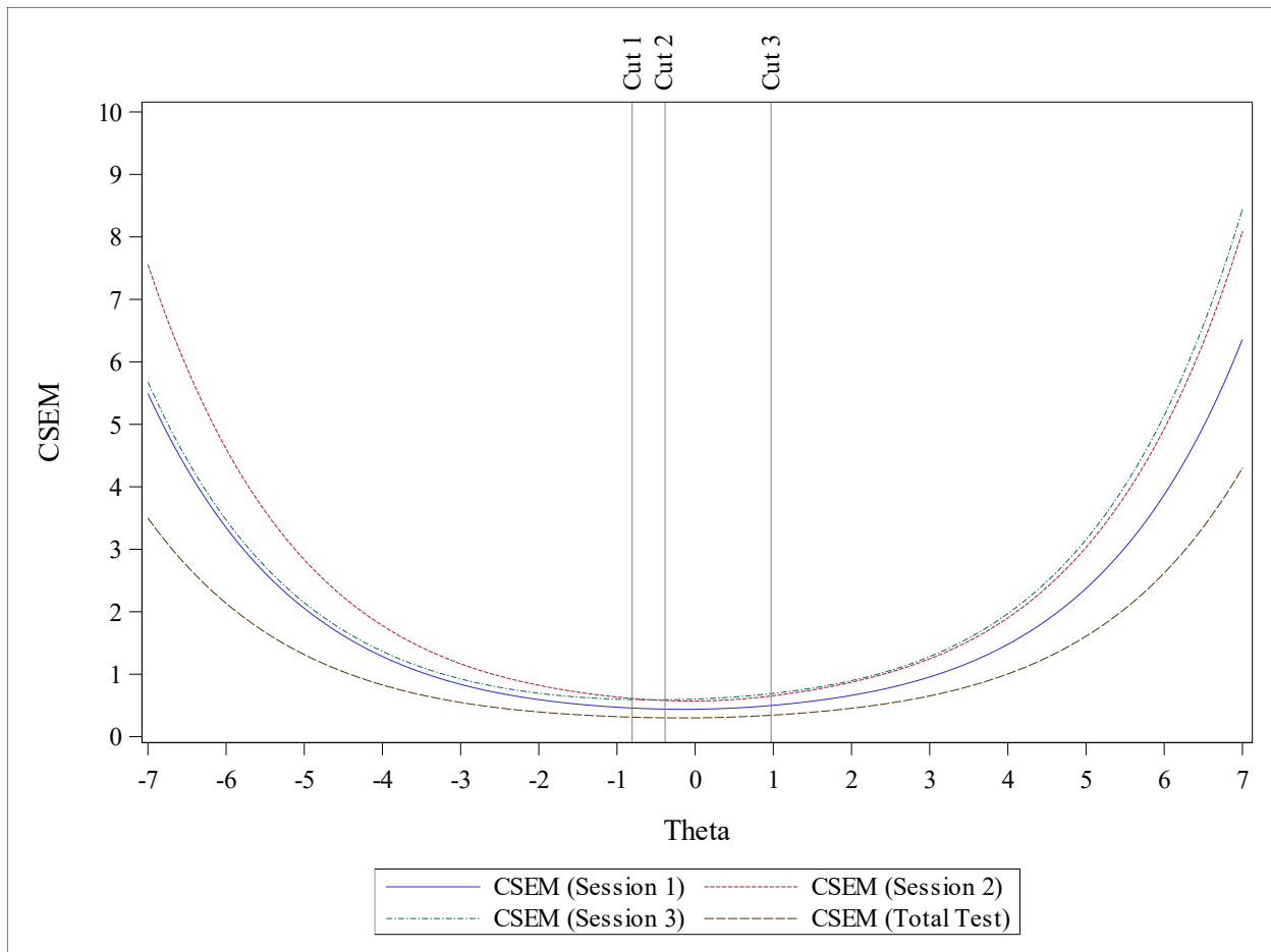
Figure 10. Grade 8 Conditional Standard Error of Measurement for 2025 Form
