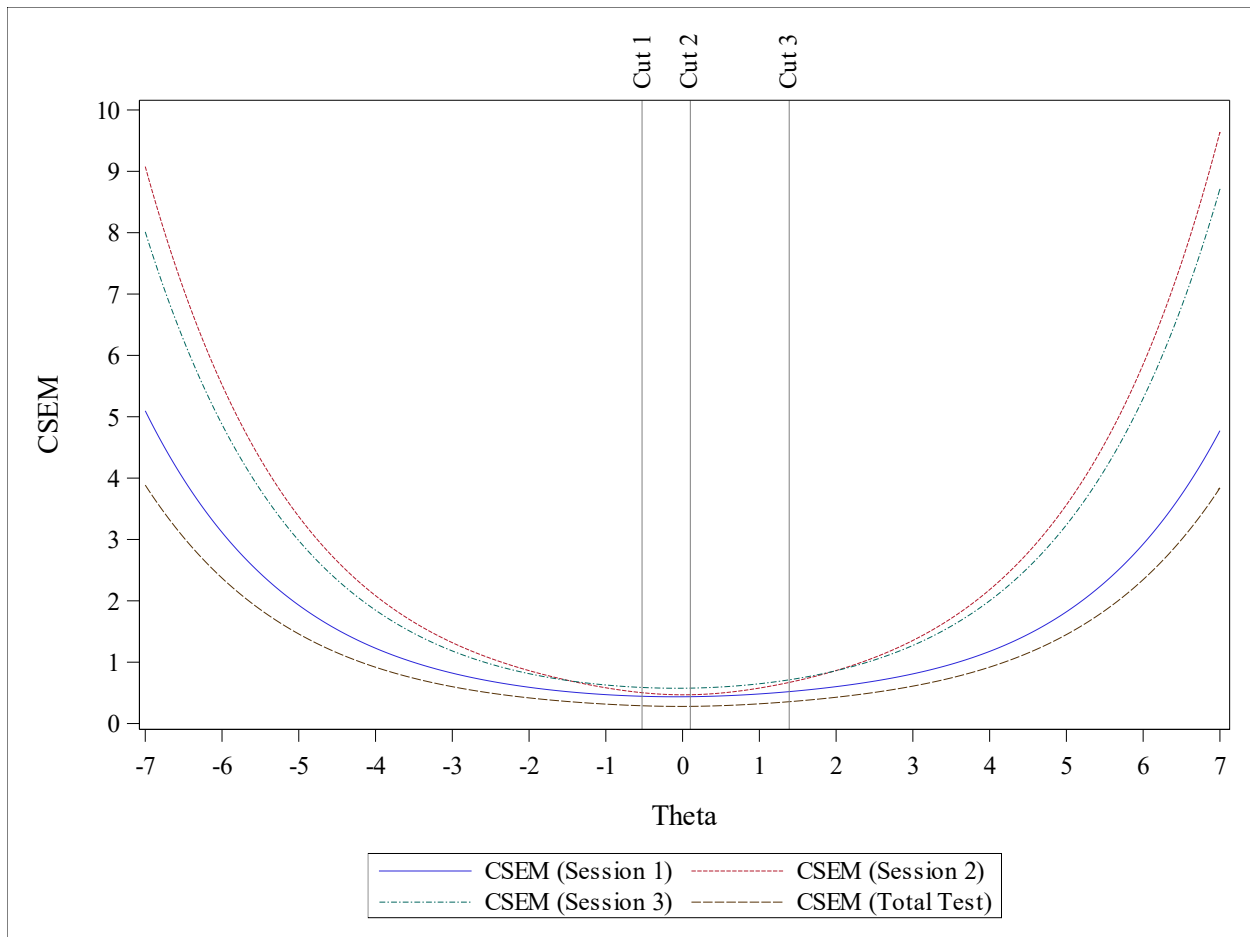
Figure 13. High School Conditional Standard Error of Measurement for 2025 Form
