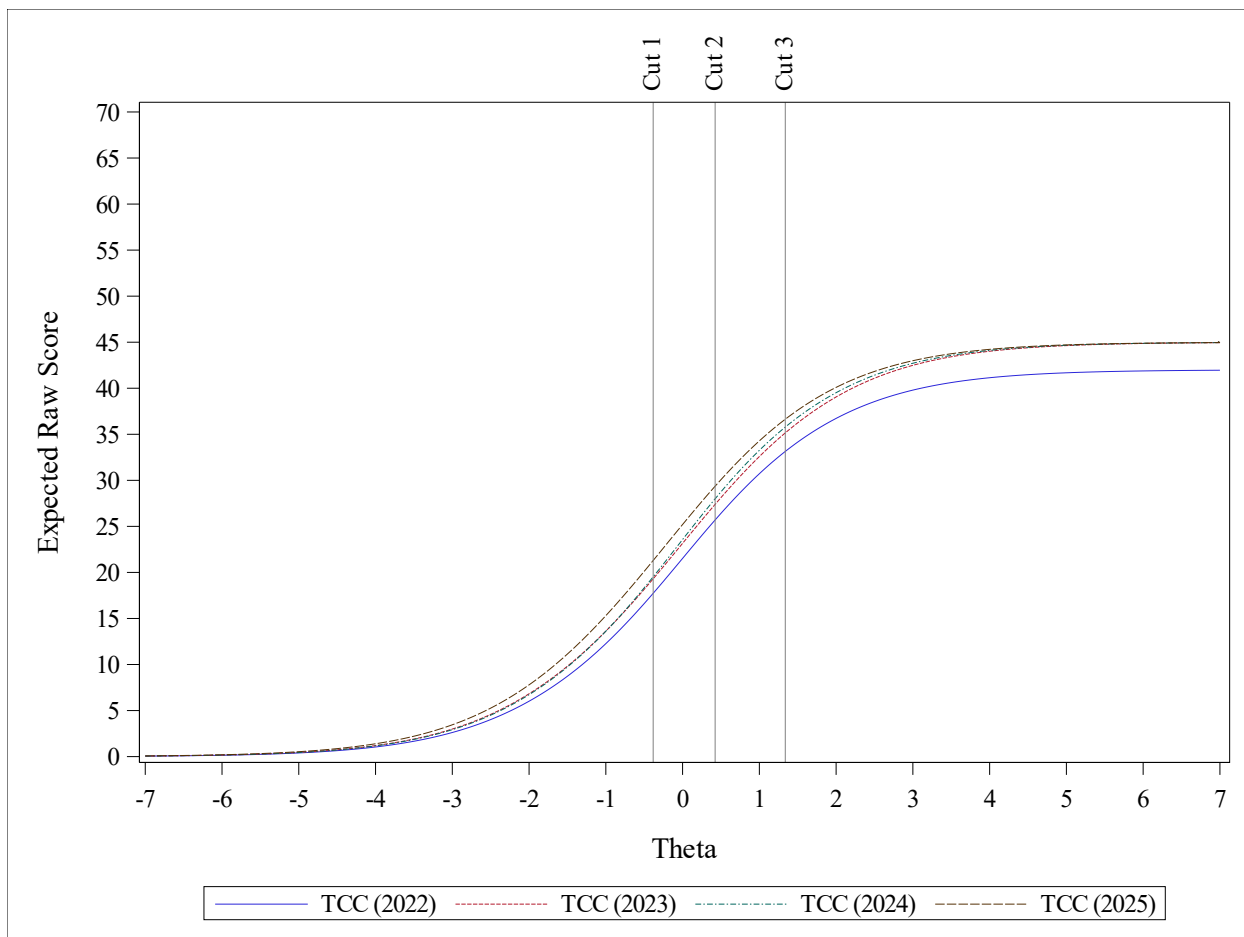
Figure 17. Grade 5 Test Characteristic Curves 2022–2025
