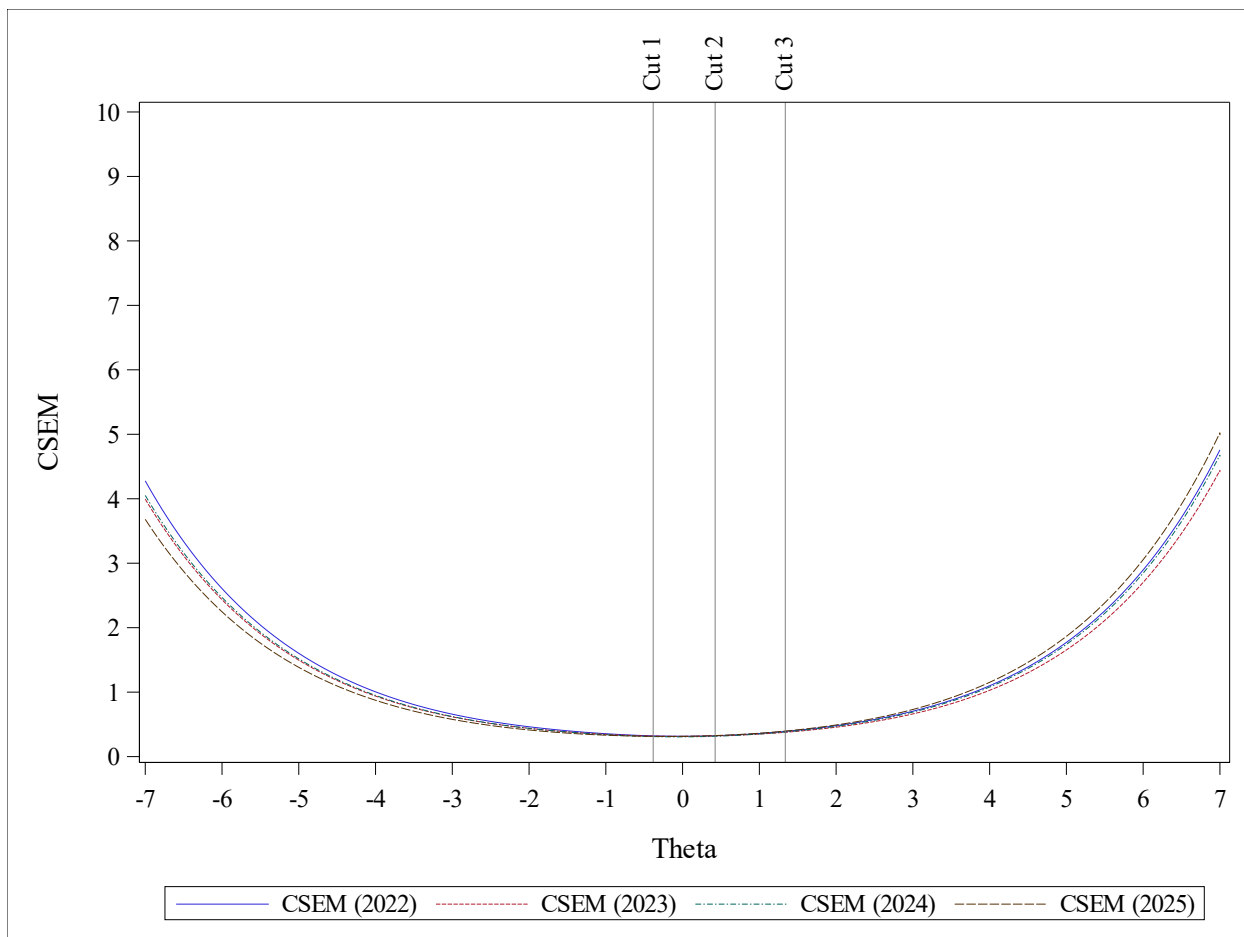
Figure 16. Grade 5 Conditional Standard Errors of Measurement 2022–2025
