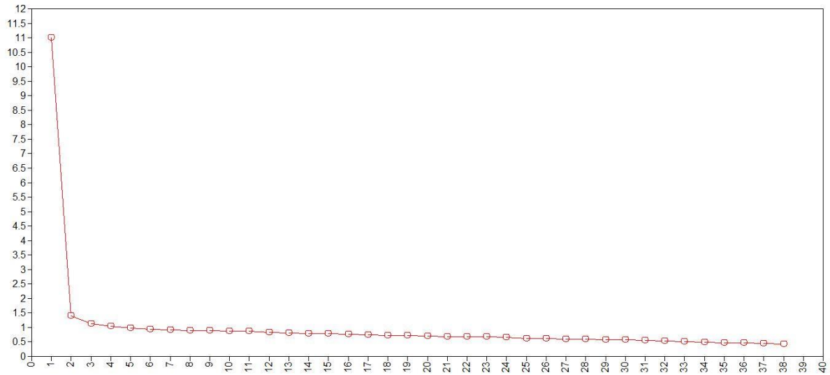
Figure 3. Grade 8 Scree Plot
