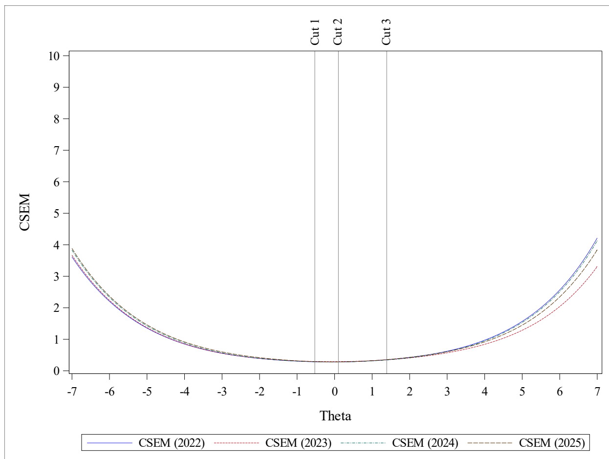
Figure 22. High School Conditional Standard Errors of Measurement 2022–2025
