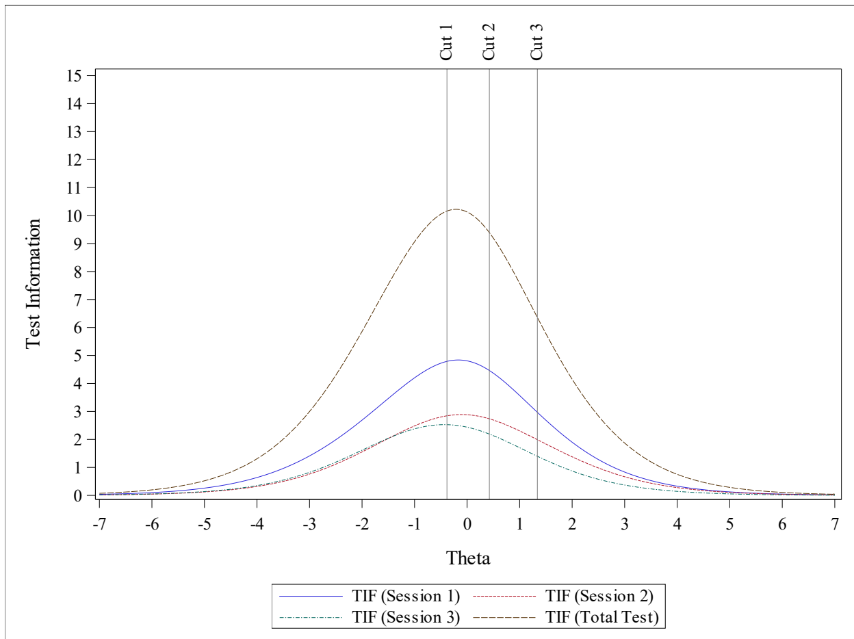
Figure 6. Grade 5 Test Information Function for 2025 Form
