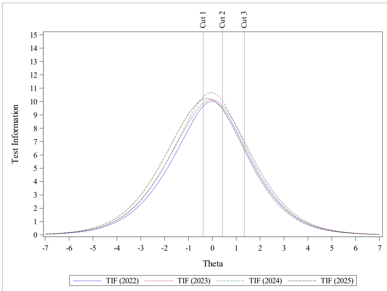
Figure 15. Grade 5 Test Information Functions 2022–2025
