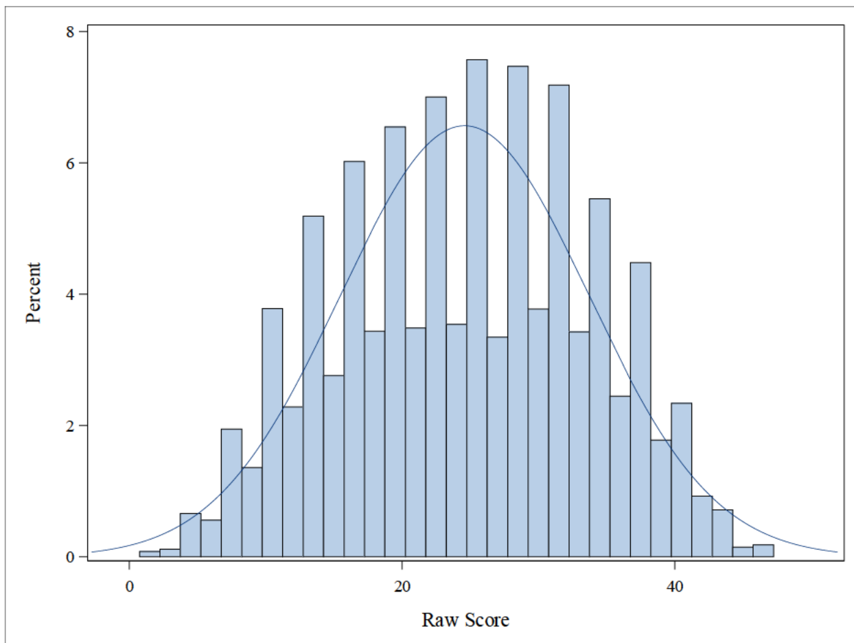
Figure 26. Grade 8 Raw Score Distribution
