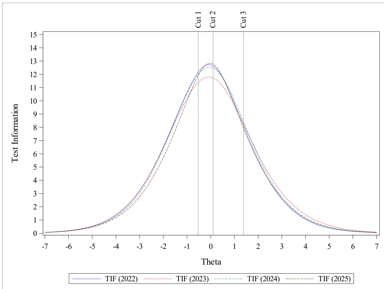
Figure 21. High School Test Information Functions 2022–2025
