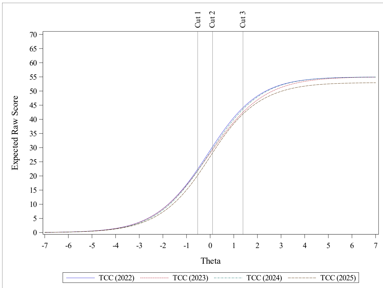
Figure 23. High School Test Characteristic Curves 2022–2025
