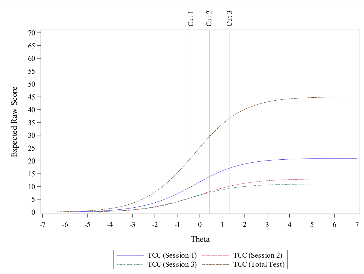
Figure 8. Grade 5 Test Characteristic Curve for 2025 Form
