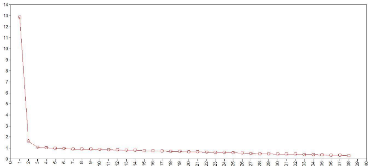
Figure 4. HS Scree Plot
