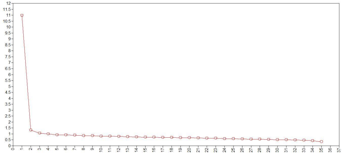
Figure 30. Grade 5 Scree Plot
