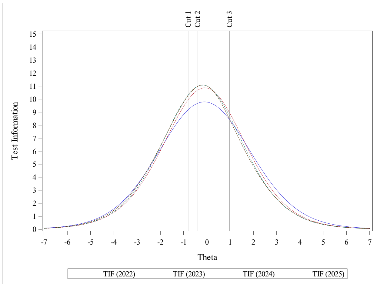
Figure 18. Grade 8 Test Information Functions 2022–2025
