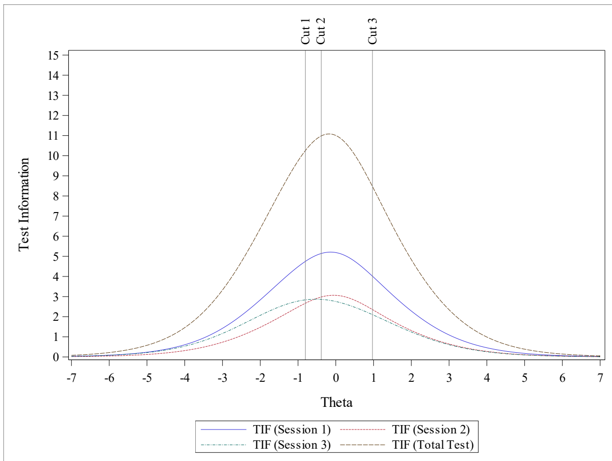
Figure 9. Grade 8 Test Information Function for 2025 Form
