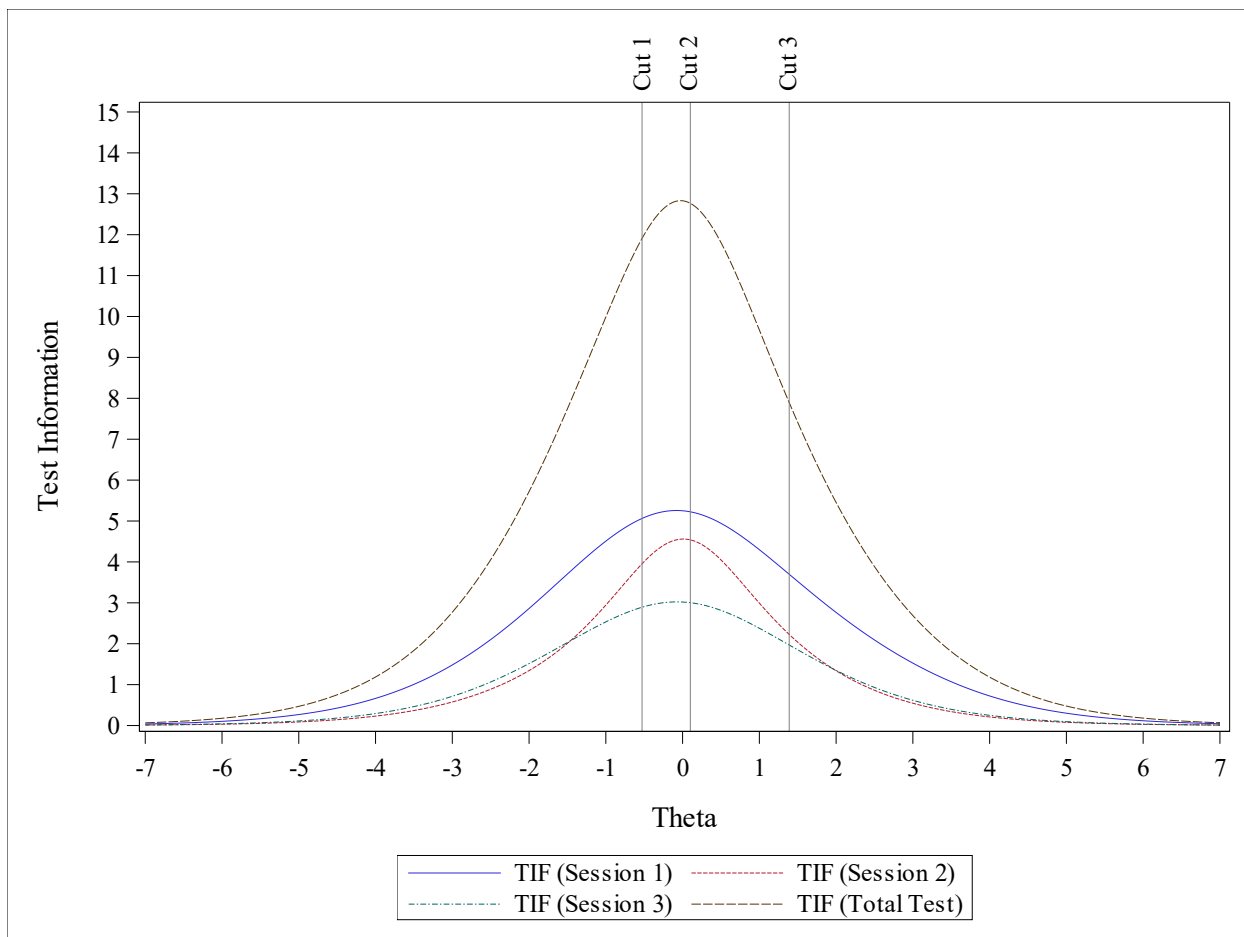
Figure 12. High School Test Information Function for 2025 Form
