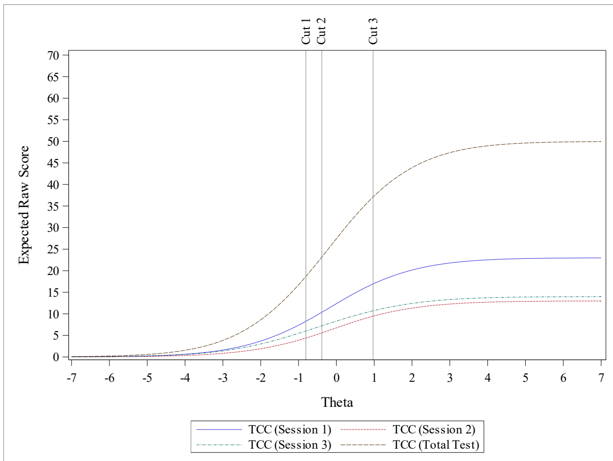
Figure 11. Grade 8 Test Characteristic Curve for 2025 Form
