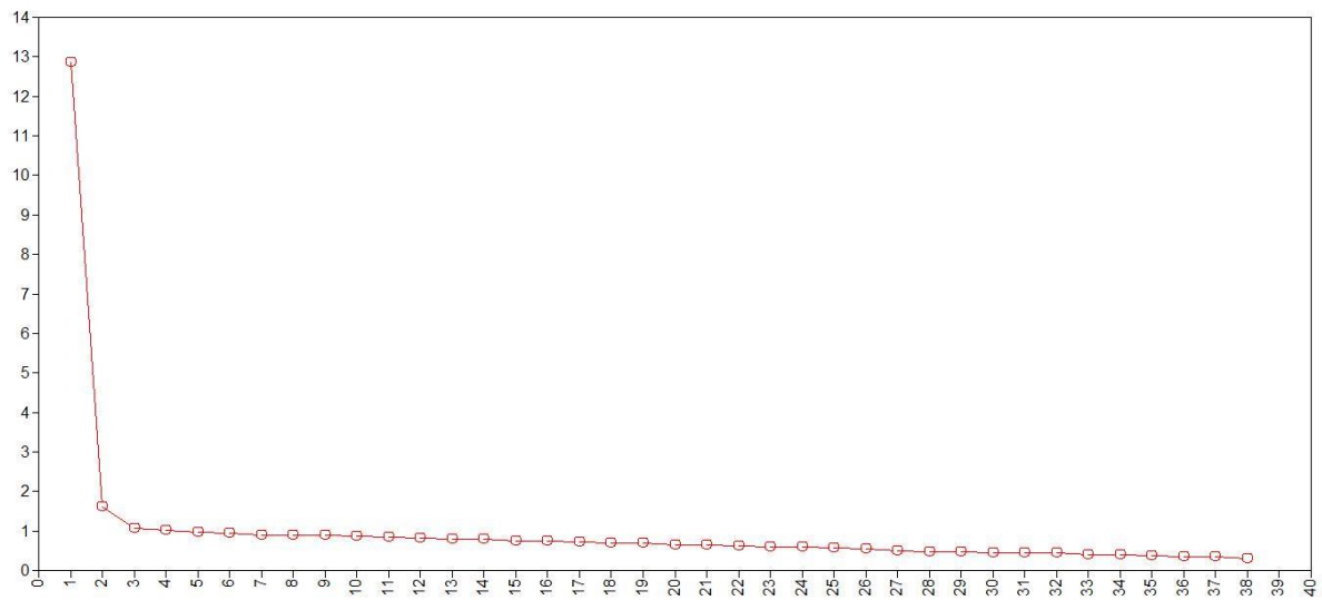
Figure 32. High School Scree Plot
