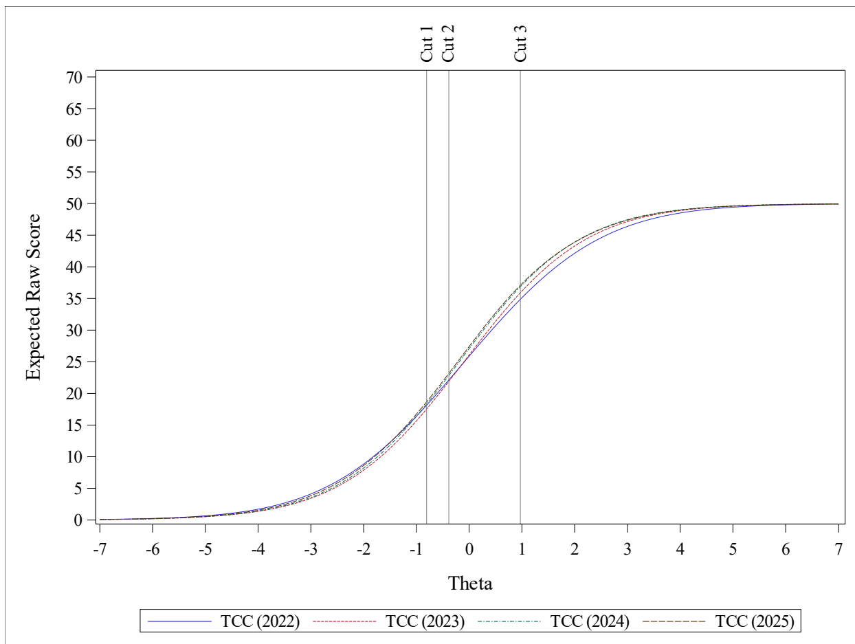
Figure 20. Grade 8 Test Characteristic Curves 2022–2025
