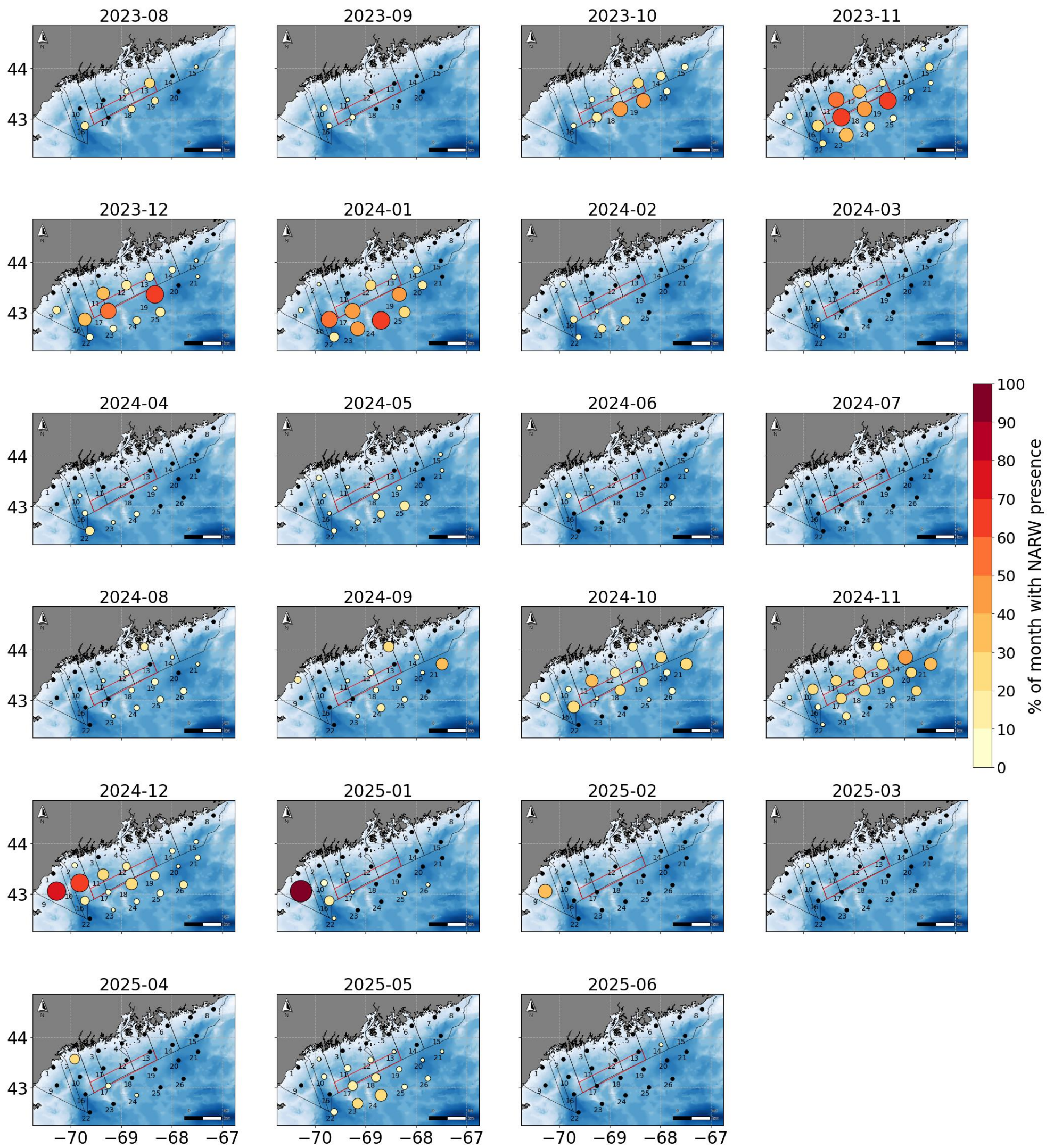
Figure S1. Preliminary results showing percent monthly presence of NARWs at all grid sites between August 2023 and June 2025. Sites are absent from monthly maps if the PAM mooring was not in the water or if the PAM mooring was not able to be recovered.
