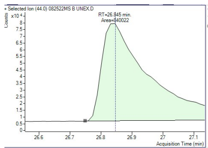
This is a limited example of peak tailing and could be caused by several factors including but not limited to: old mobile phases, old column guard cartridge, old column, overloading of the column, interfering coelutions. If the issue is gross and persistent troubleshooting of the instrument may be required.
