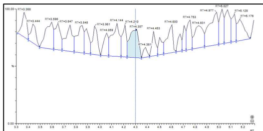
This is an example of baseline noise as there are no definite peaks that distinguish themselves from the baseline and the 'peak' at the expected retention time has a signal to noise ratio of <3.
