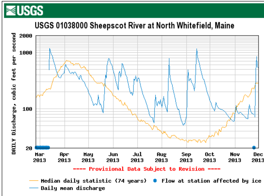
Figure 1. Sheepscot River flows for 2013 measured in North Whitefield, Maine as recorded by the USGS stream gauge. Actual flows for 2013 are in blue, while the 74 year median is in orange. Ice cover in March and November is indicated by dark blue dots.
