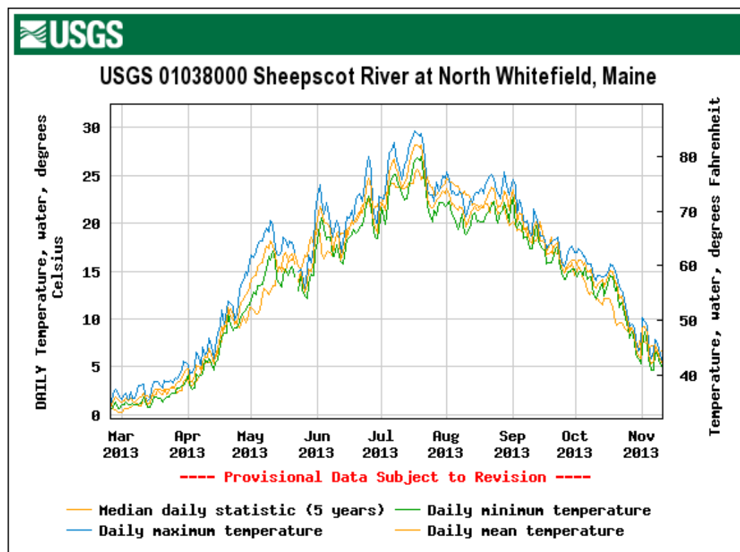
Figure 2. Daily water temperature for the Sheepscot River from the USGS gauge in Whitefield. Maximum, minimum and daily means are presented in blue, green and orange respectively. The 5-year median water temperature is the lower orange line.
