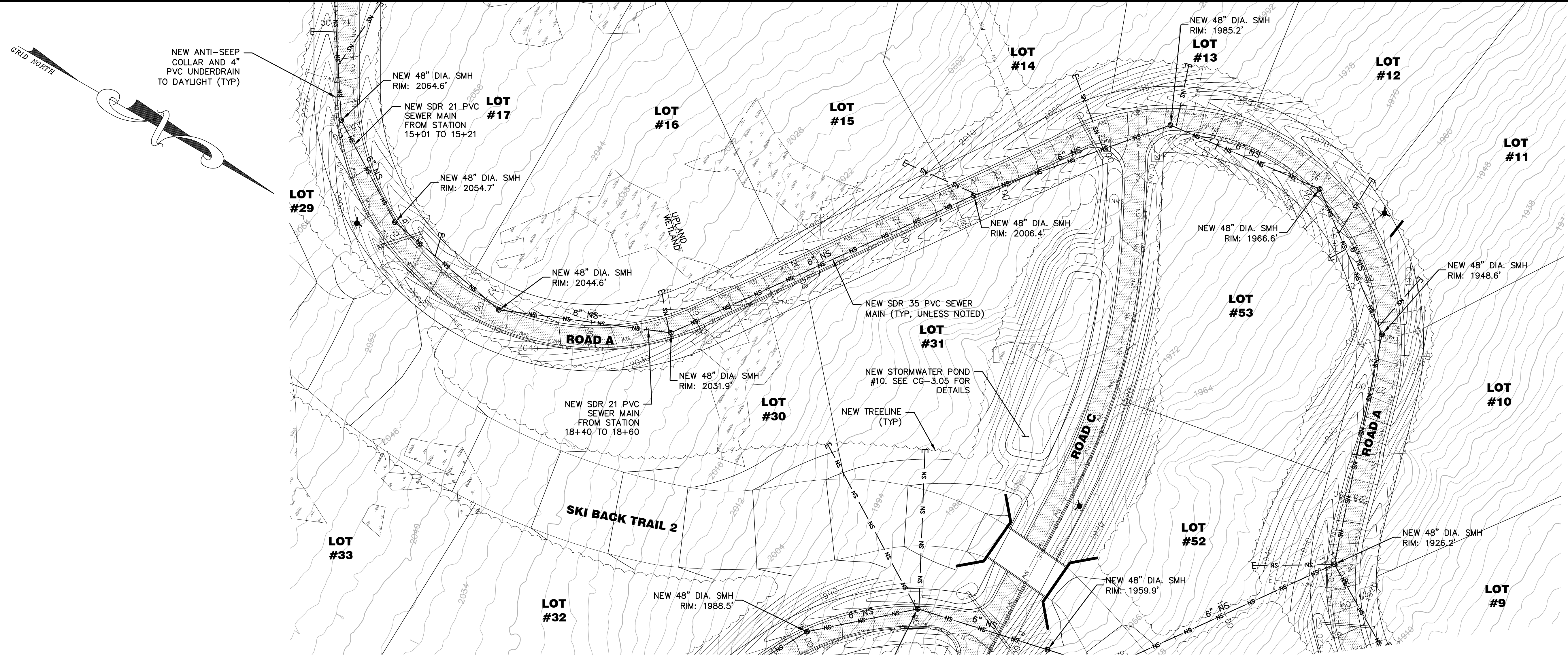
SEWER PLAN 15+00 TO 28+00 SCALE: 1"=50'
