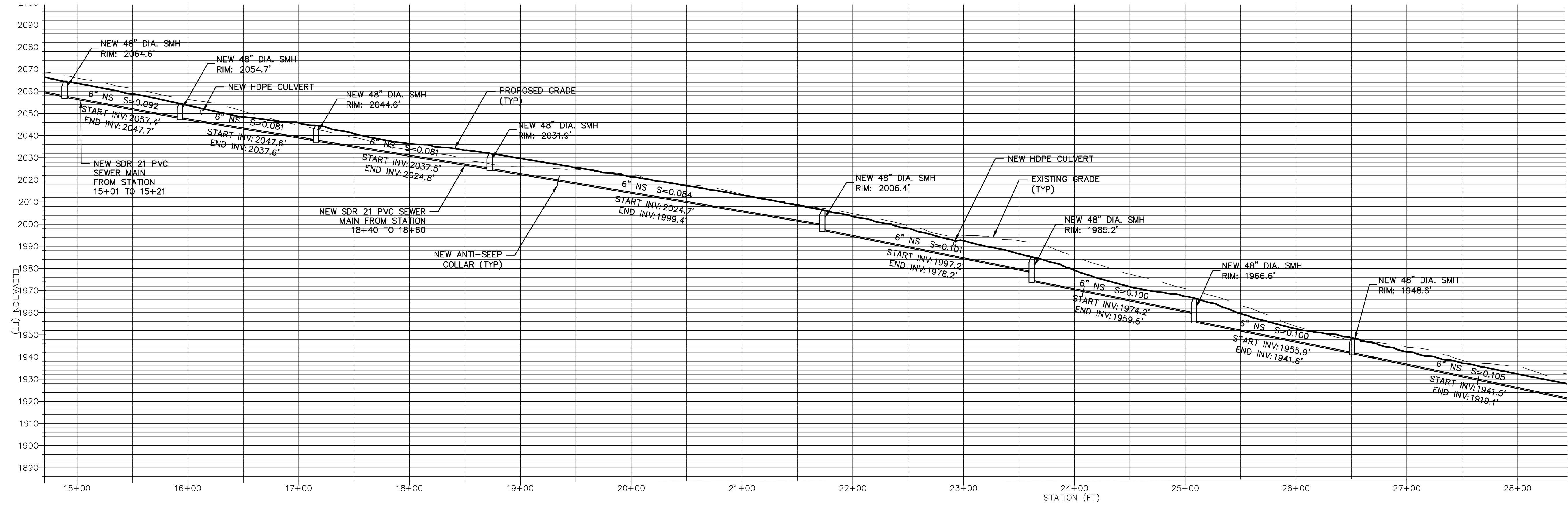
SEWER PROFILE 15+00 TO 28+00 HORIZONTAL SCALE 1" = 50' VERTICAL SCALE 1" = 25'
