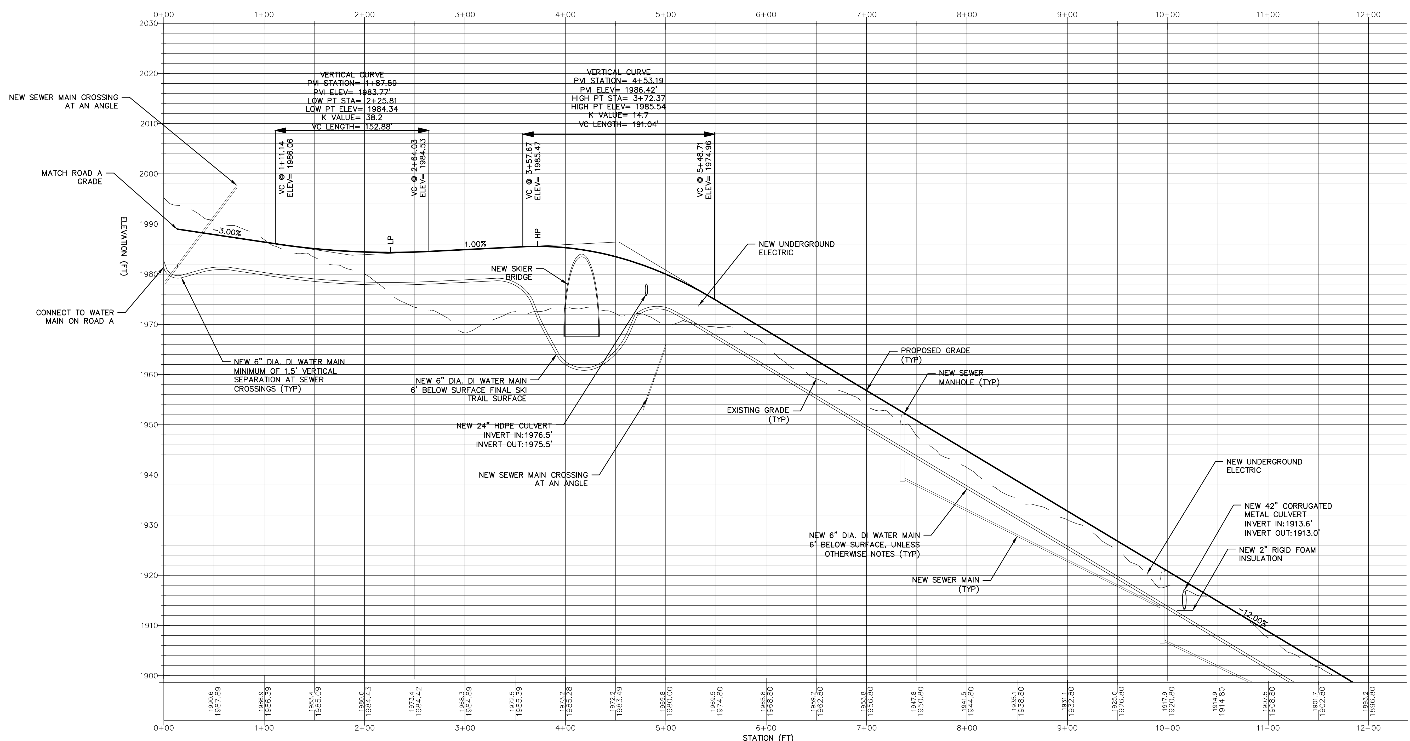
C ROAD PROFILE 0+00 TO 9+00 HORIZONTAL SCALE 1" = 50' VERTICAL SCALE 1" = 10'
