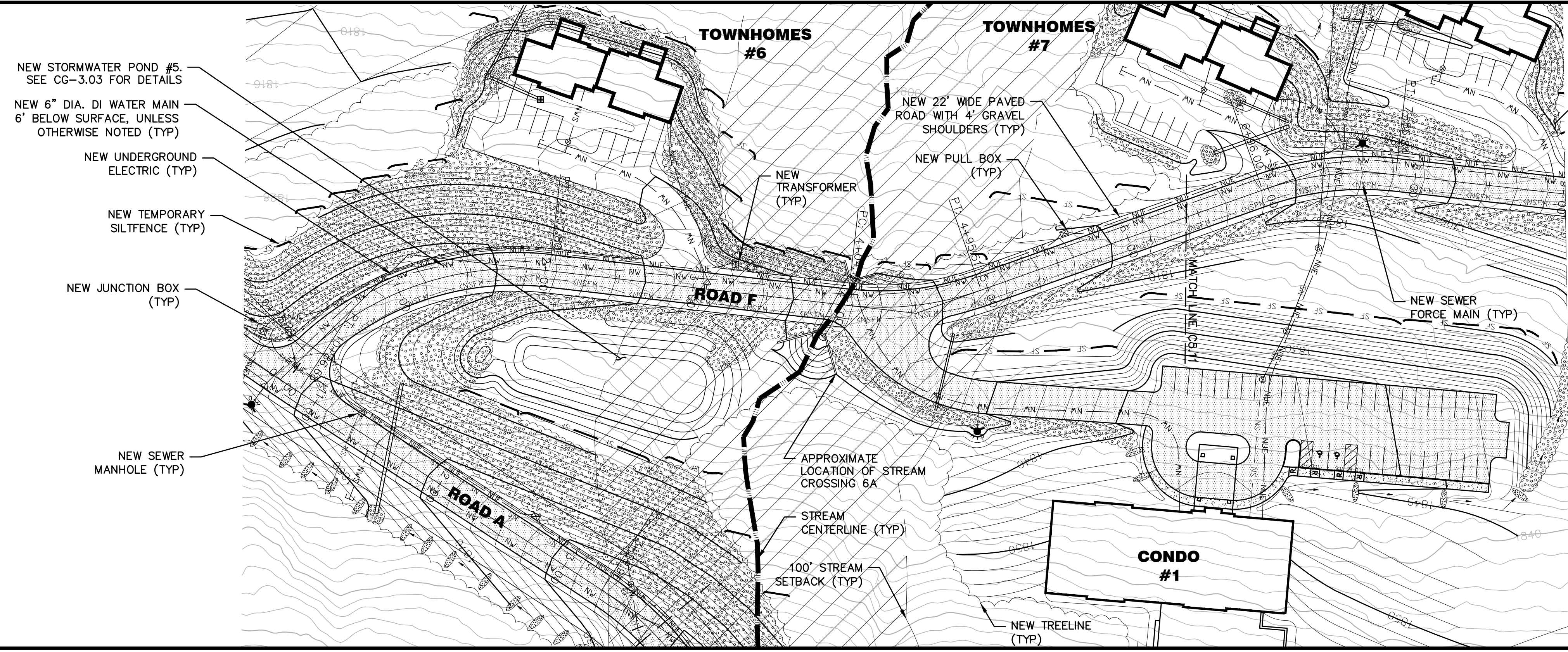
F ROAD PLAN 0+00 TO 8+00 SCALE: 1"=50'
