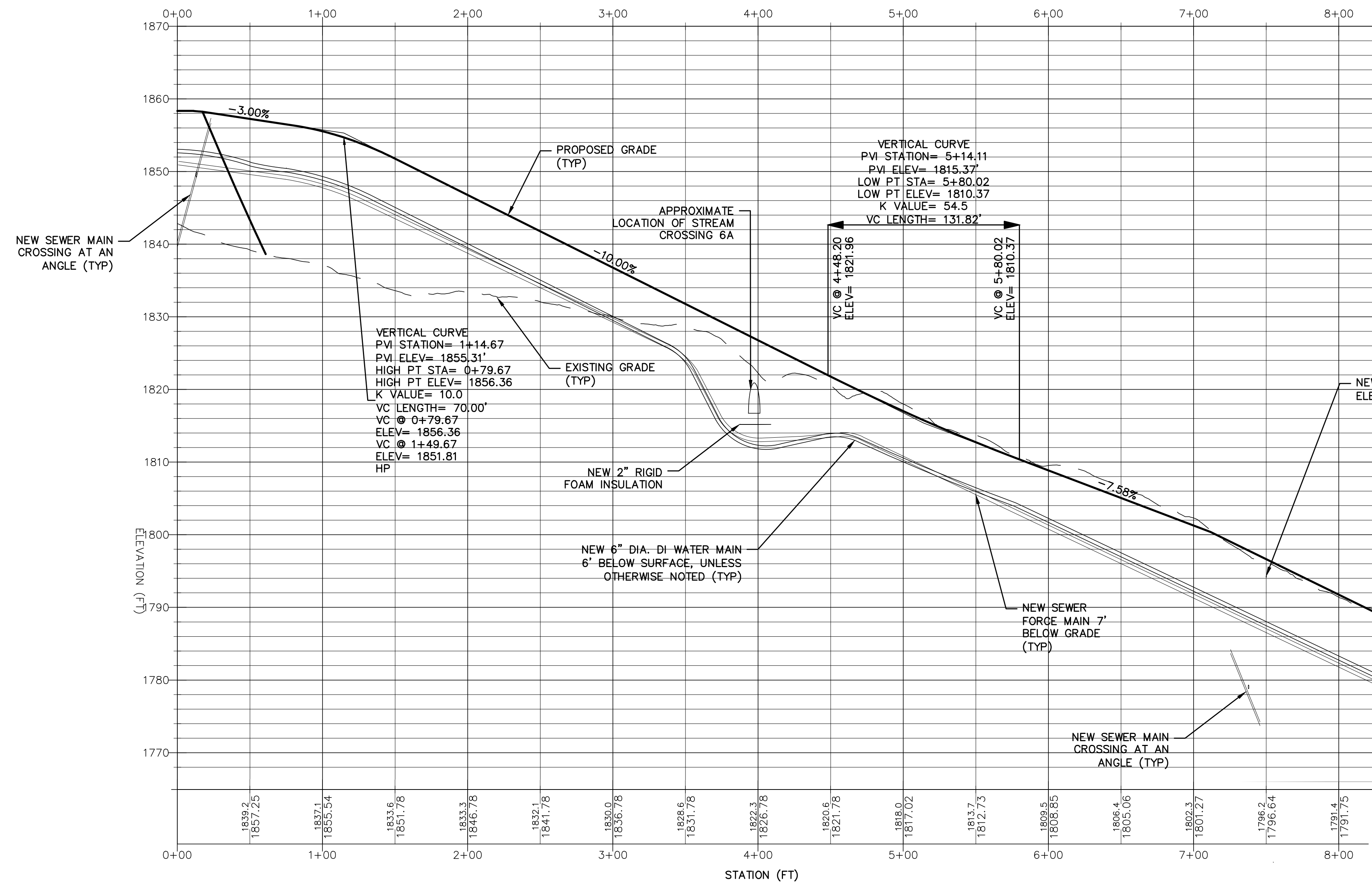
F ROAD PROFILE 0+00 TO 8+00 HORIZONTAL SCALE 1" = 50' VERTICAL SCALE 1" = 10'
