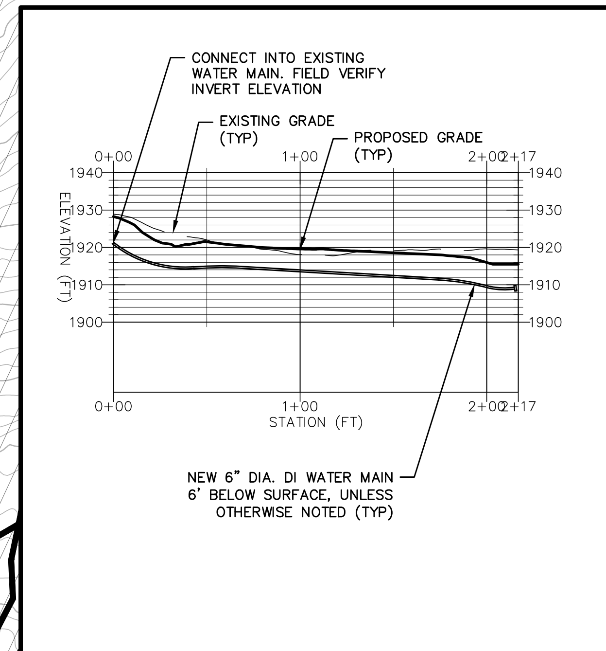
B2 WATER MAIN PROFILE HORIZONTAL SCALE 1" = 50' VERTICAL SCALE 1" = 25'
