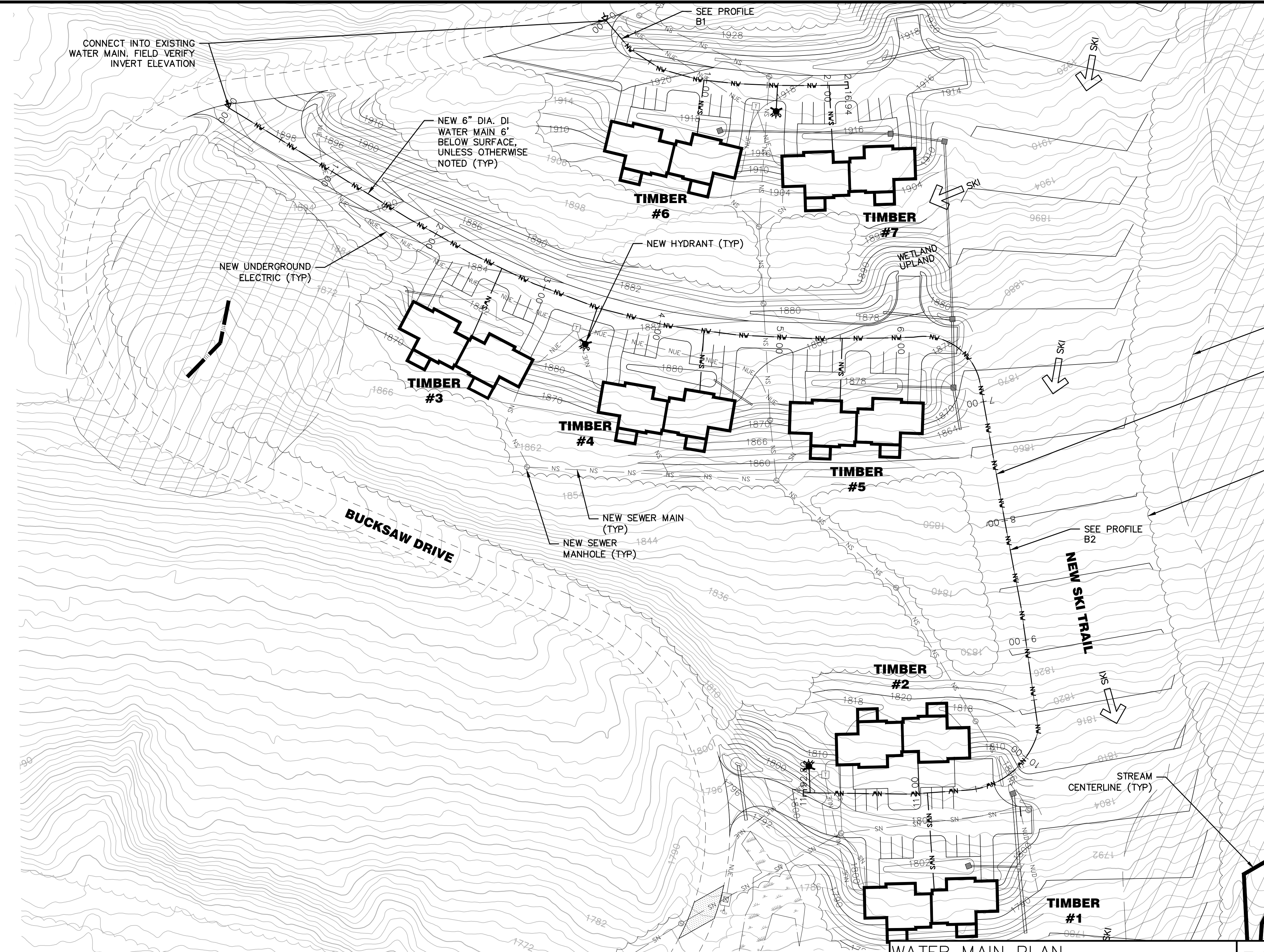
WATER MAIN PLAN SCALE: 1"=50'
