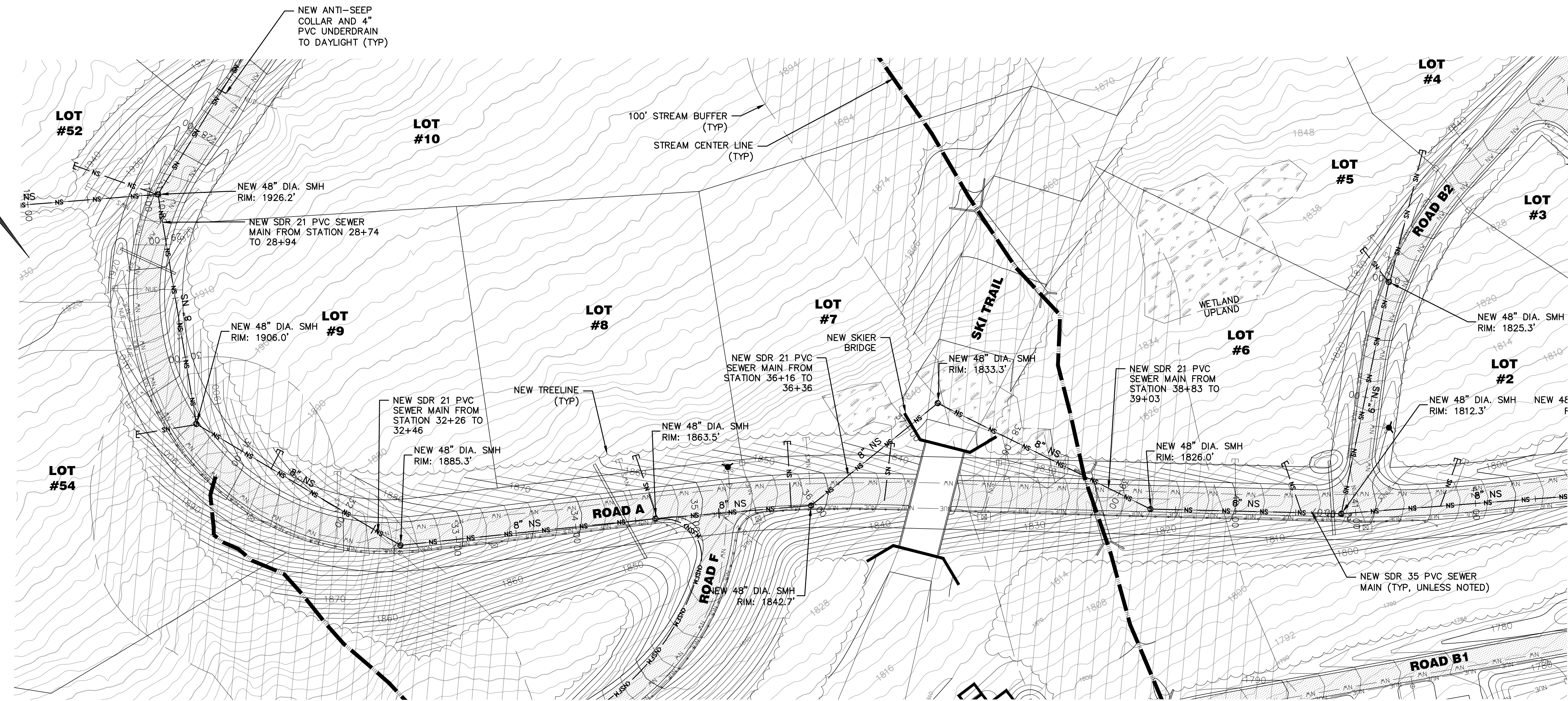
SEWER PLAN 28+00 TO 42+00 SCALE: 1"=50'
