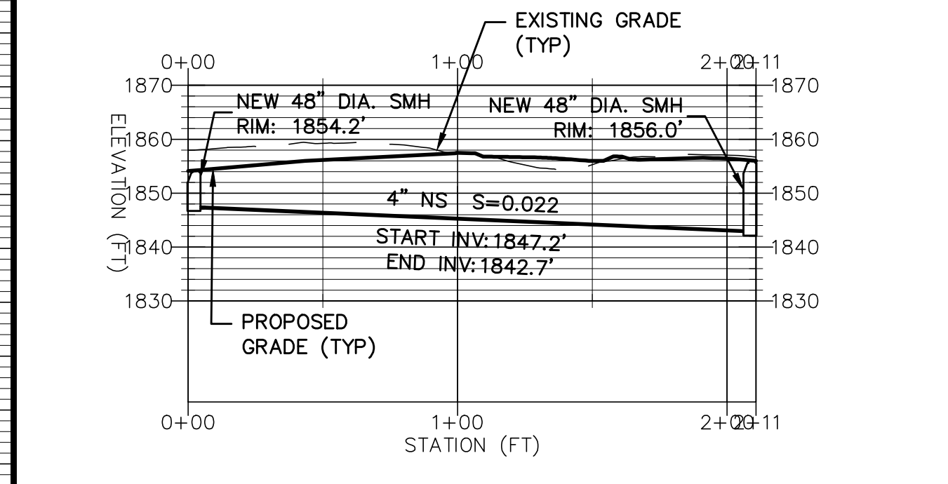
SEWER PROFILE SPUR B1 HORIZONTAL SCALE 1" = 50' VERTICAL SCALE 1" = 25'
