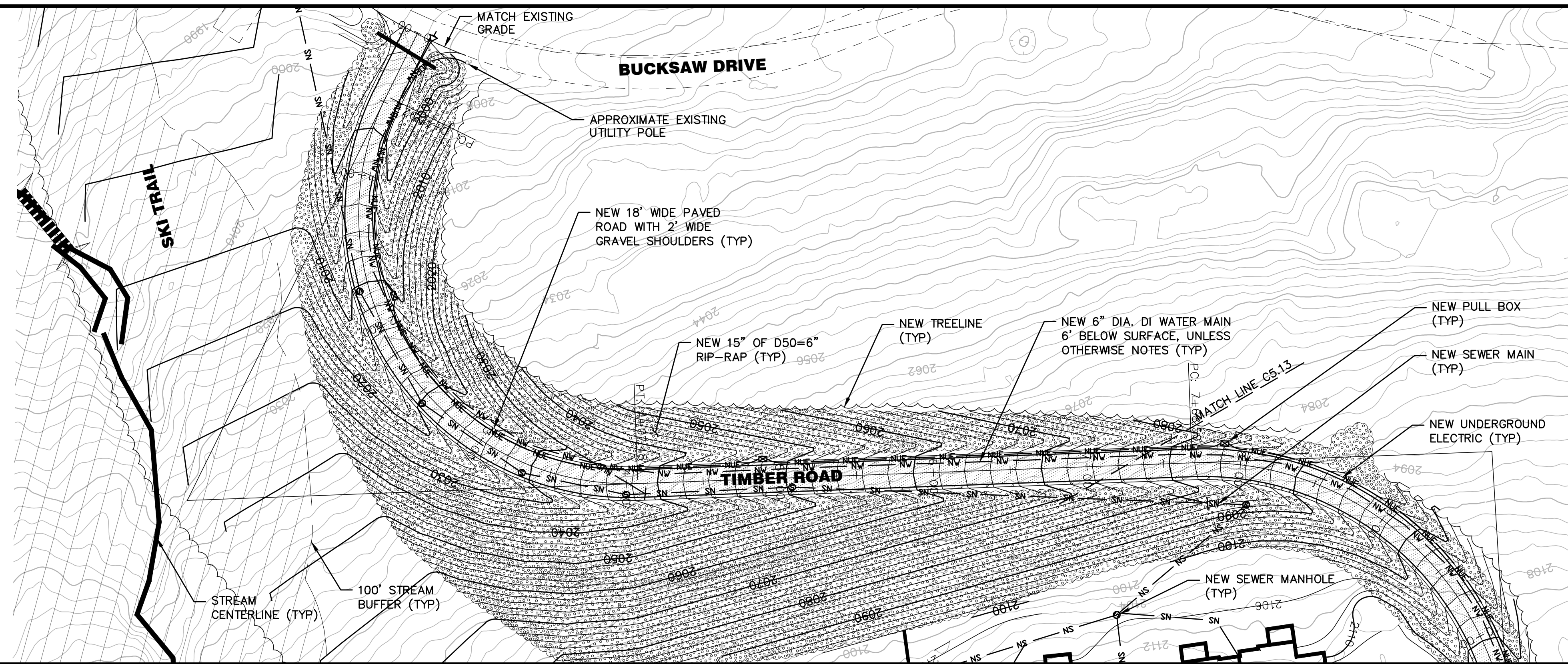
TIMBER ROAD PLAN 0+00 TO 8+00 B1 SCALE: 1"=50'
