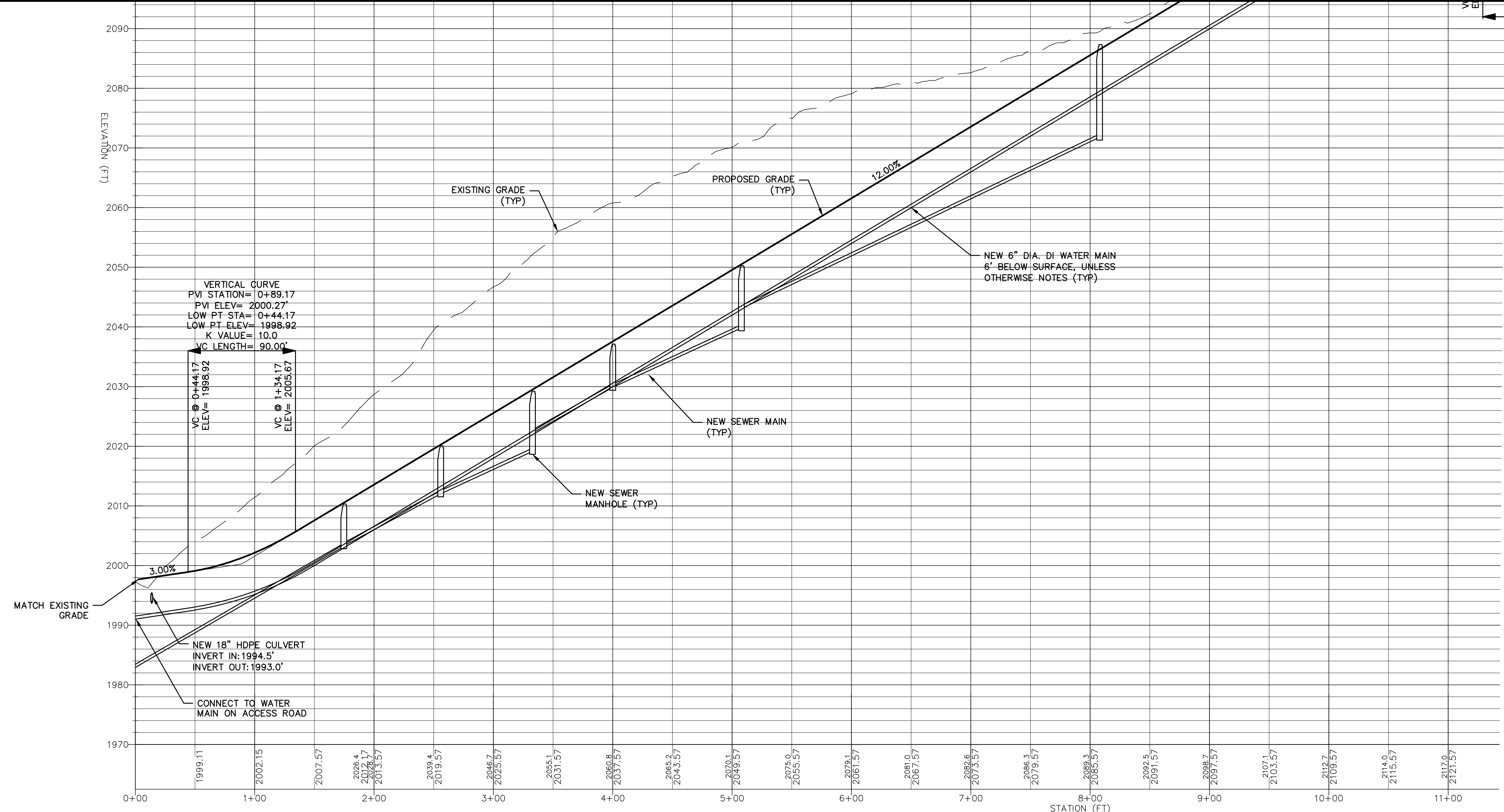
TIMBER ROAD PROFILE 0+00 TO 8+00 A1 HORIZONTAL SCALE 1" = 50' VERTICAL SCALE 1" = 10'
