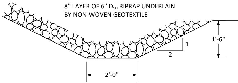
RIPRAP CHANNEL DETAIL NTS
