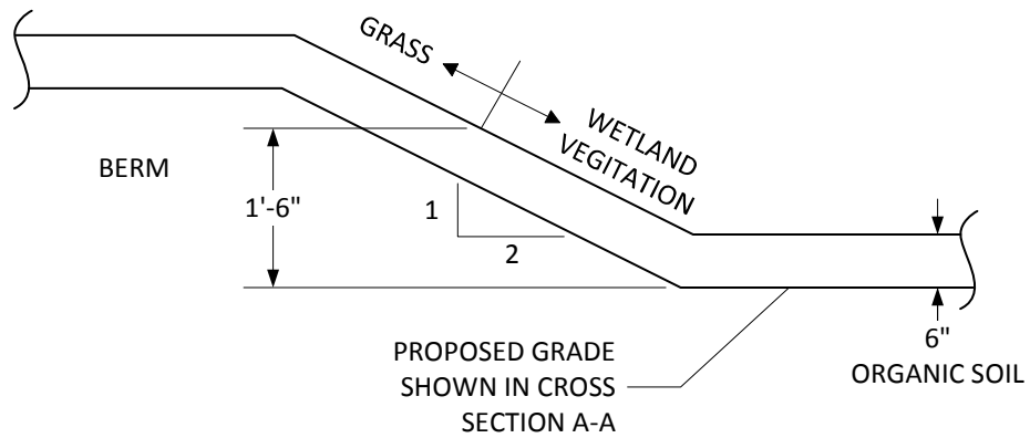
VEGETATION AND WETLAND SUBSTRATE DETAIL NTS
