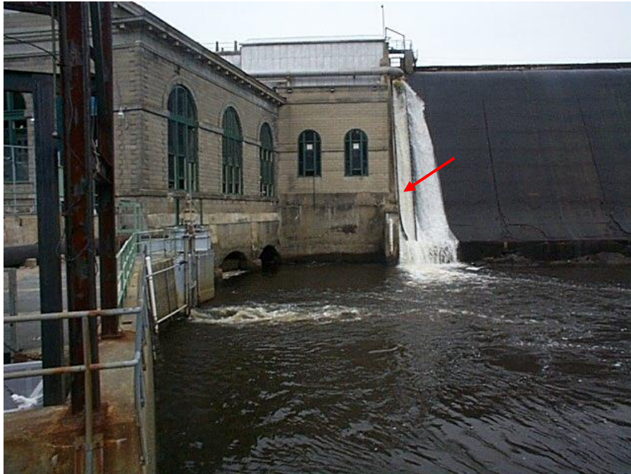
FIGURE 5 VIEW OF DISCHARGE FROM DOWNSTREAM FISH PASSAGE PIPE AND SURFACE WEIR AT THE ELLSWORTH DAM
