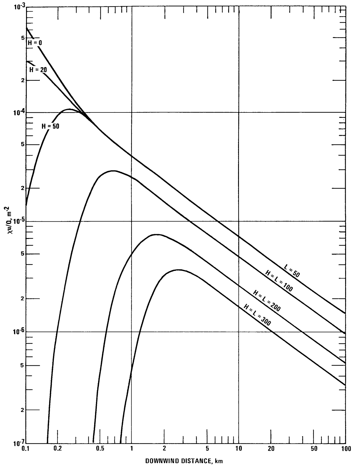
Figure 4-1 2.^^^ Document Error r^^^ Document Error r^^^ Stability class D, urban terrain; u/Q vs. distance for various plume heights (H), assuming very restrictive mixing heights (L); L = 50m for H ≤ 50m; L = H for H > 50m.
