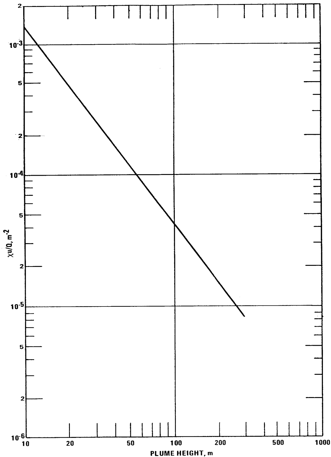
Figure 4-1. Maximum \chi u/Q as a function of plume height, H (for use only with the simple screening procedure).
