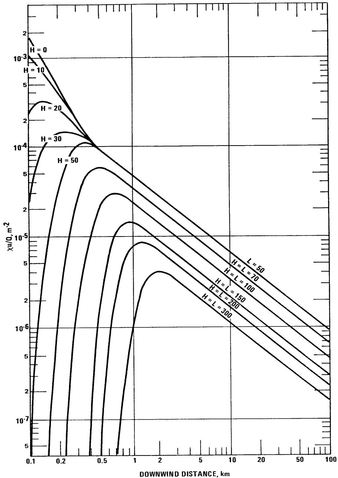
Figure 4-5. \chi u/Q vs. distance for various plume heights (H), assuming very restrictive mixing heights (L); L = 50m for H ≤ 50m; L = H for H > 50m.
