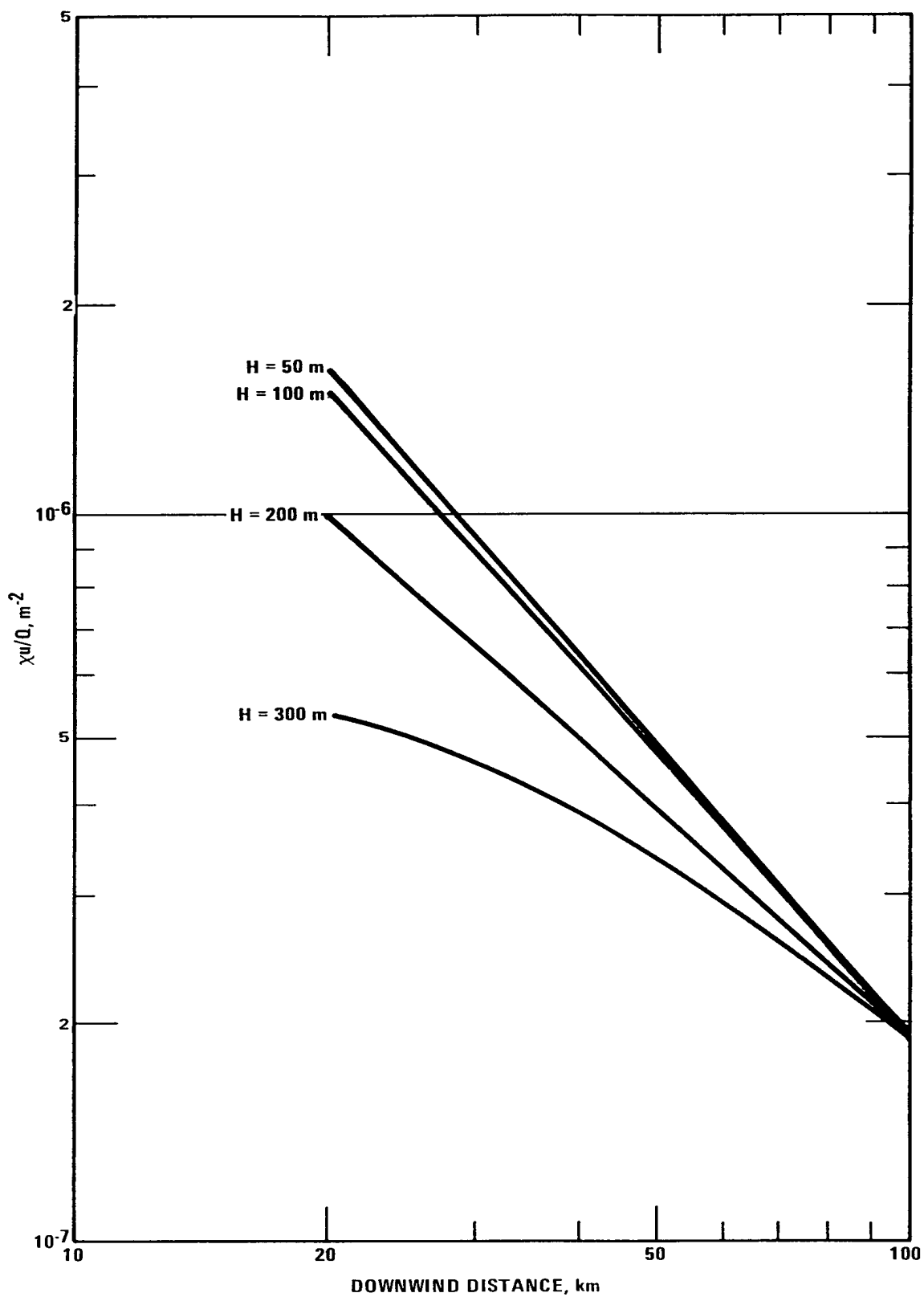
Figure 4-19. Maximum \chi u/Q as a function of downwind distance and plume height (H), assuming a mixing height of 500m; D stability.
