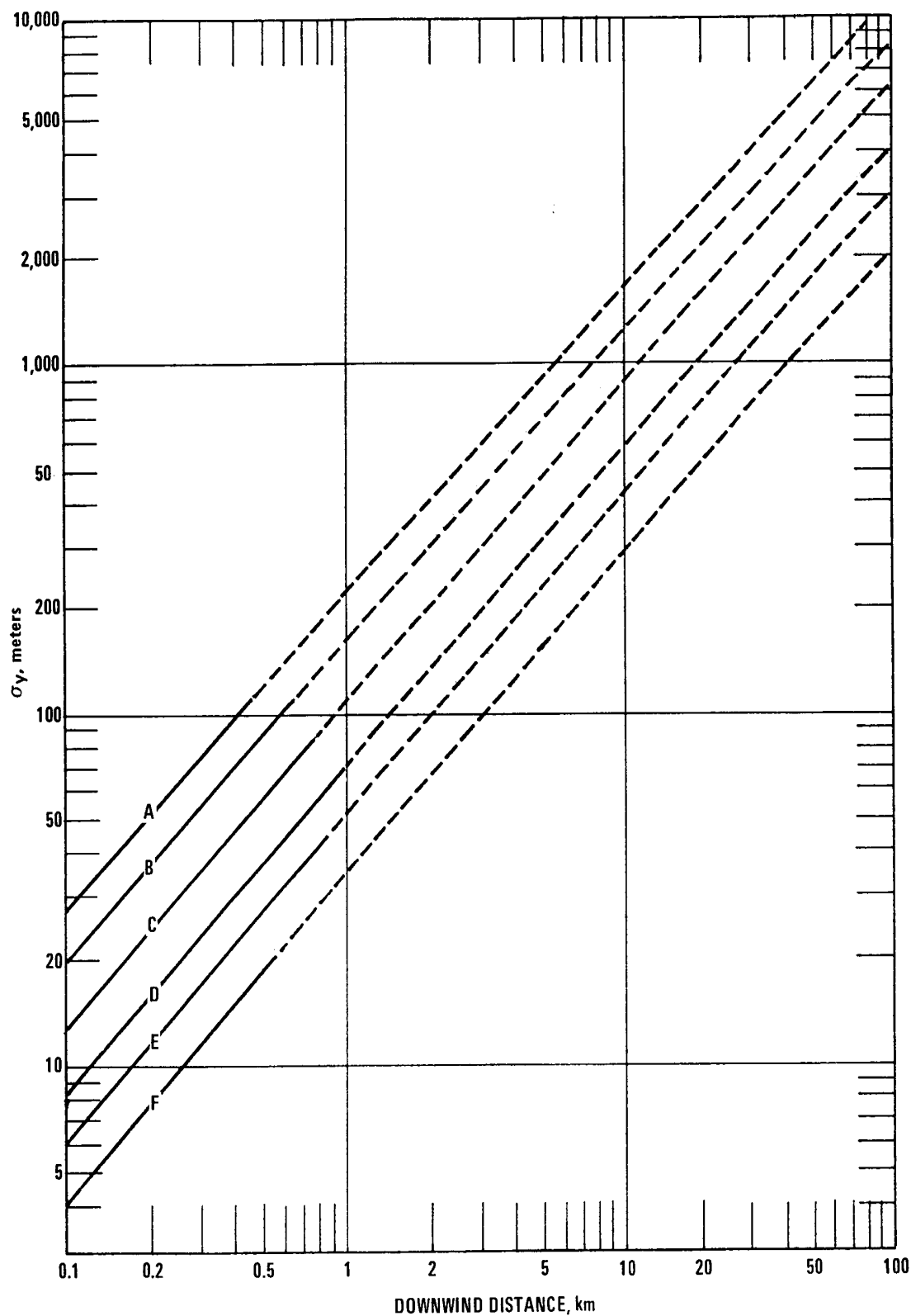
Figure 4-1 8.^^^D ocmnt E r r o r^^^^ ^Doc- ument E r r o r^^^Hor izontal disper- sion param- eter ( \sigma_y ) as a function of down- wind distance and stability class; rural terrain.
