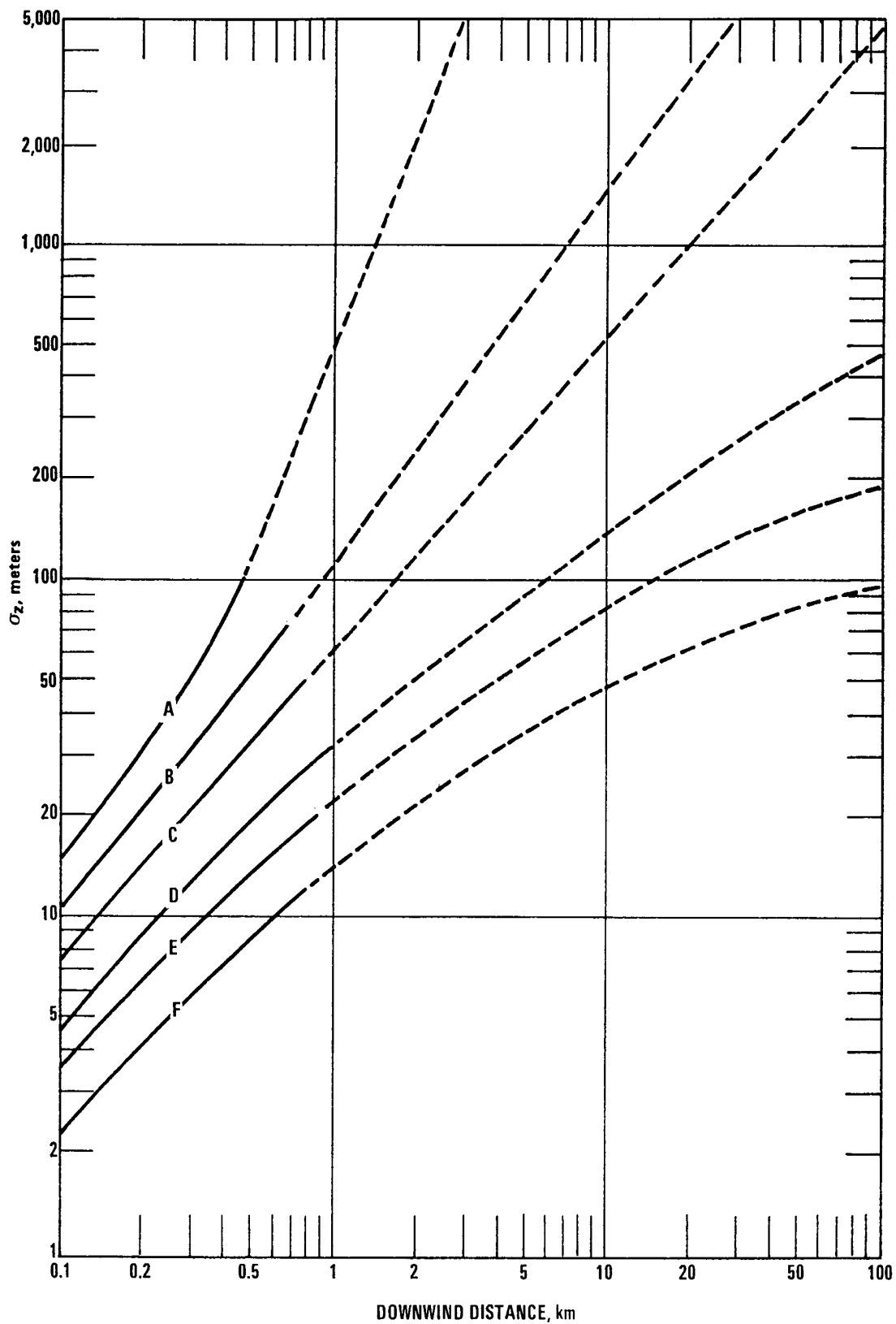
Figure 4-1 4.^^^ Docu- ment E r r o r^^^ Doc ^^Doc ument E r r o r^^^Ve rtical disper- sion parame- ter ( \sigma_z ) as a func- tion of down- wind dis- tance and stability class; rural terrain.
