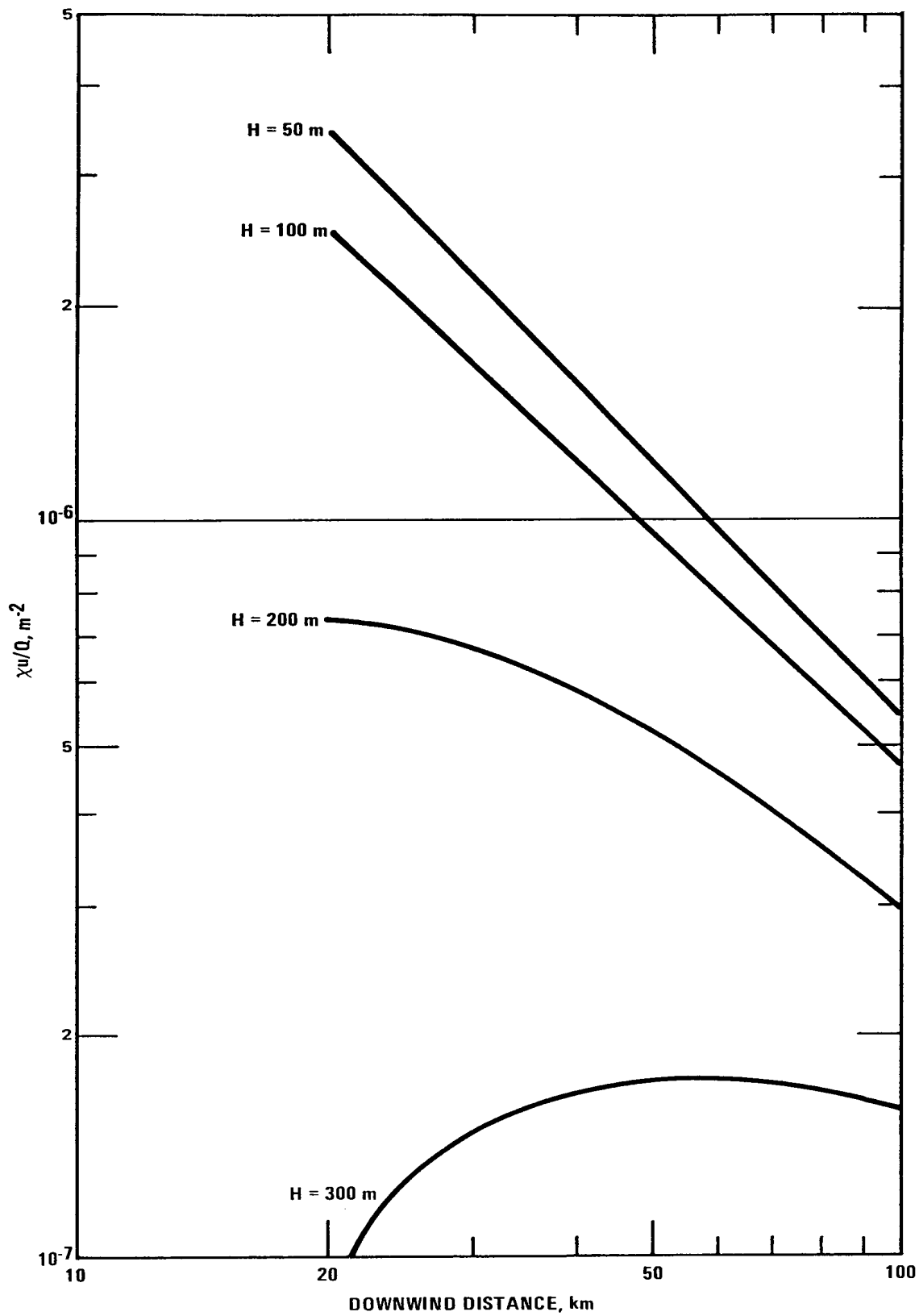
Figure 4-20. Maximum \chi u/Q as a function of downwind distance and plume height (H); E stability.
