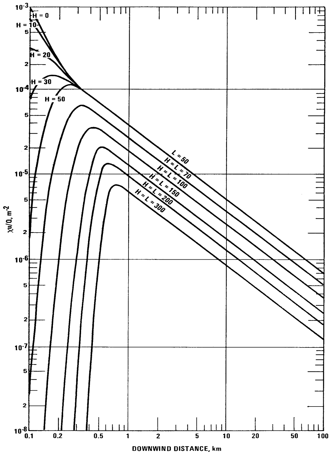
Figure 4-4. \chi u/Q vs. distance for various plume heights (H), assuming very restrictive mixing heights (L); L = 50m for H \leq 50 m; L = H for H > 50 m.
