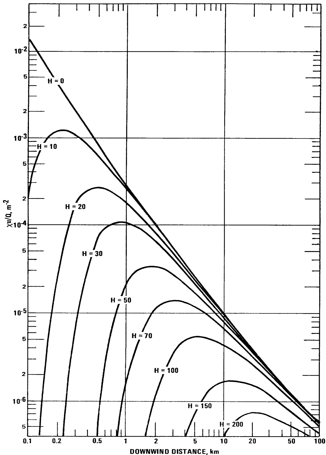
Figure 4-8. \chi u/Q vs. distance for various plume heights (H), assuming very restrictive mixing heights (L); L = 50m for H ≤ 50m; L = H for H > 50m.
