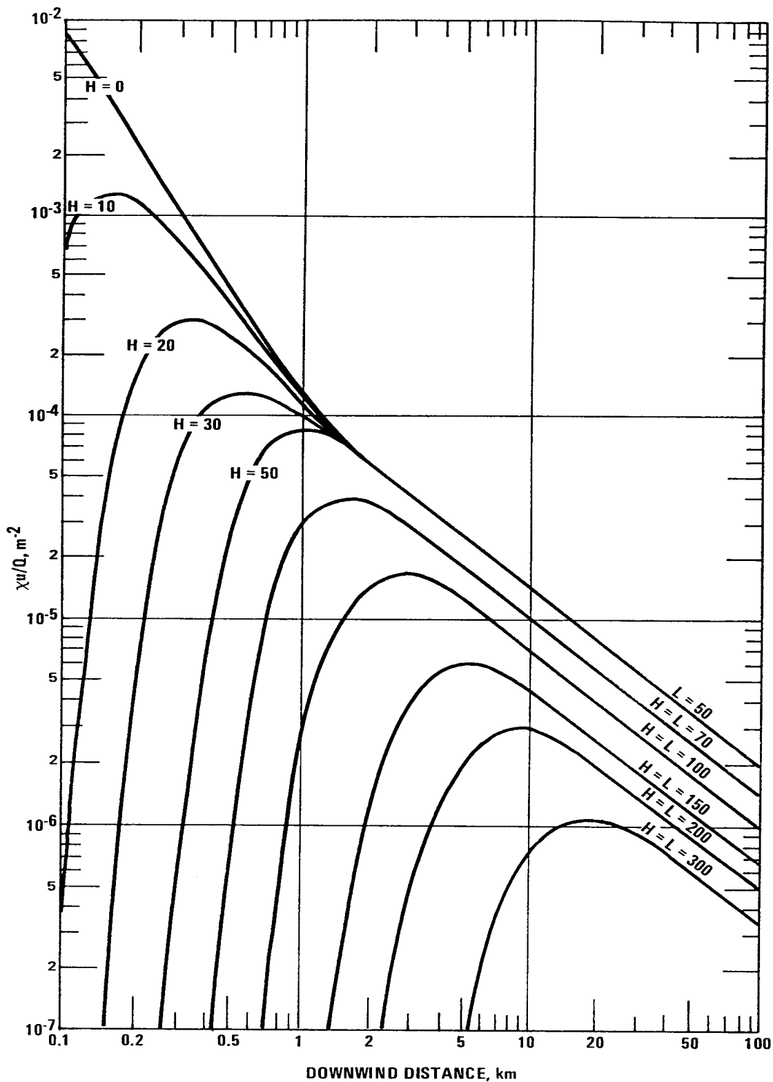
Figure 4-7. Stability class D, rural terrain; \chi u/Q vs. distance for various plume heights (H), assuming very restrictive mixing heights (L); L = 50m for H \leq 50 m; L = H for H > 50 m.
