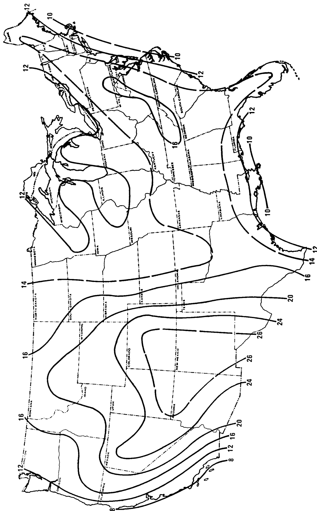
Figure 4-15. Isopleths (hundredths of meters) of mean annual afternoon mixing heights.
