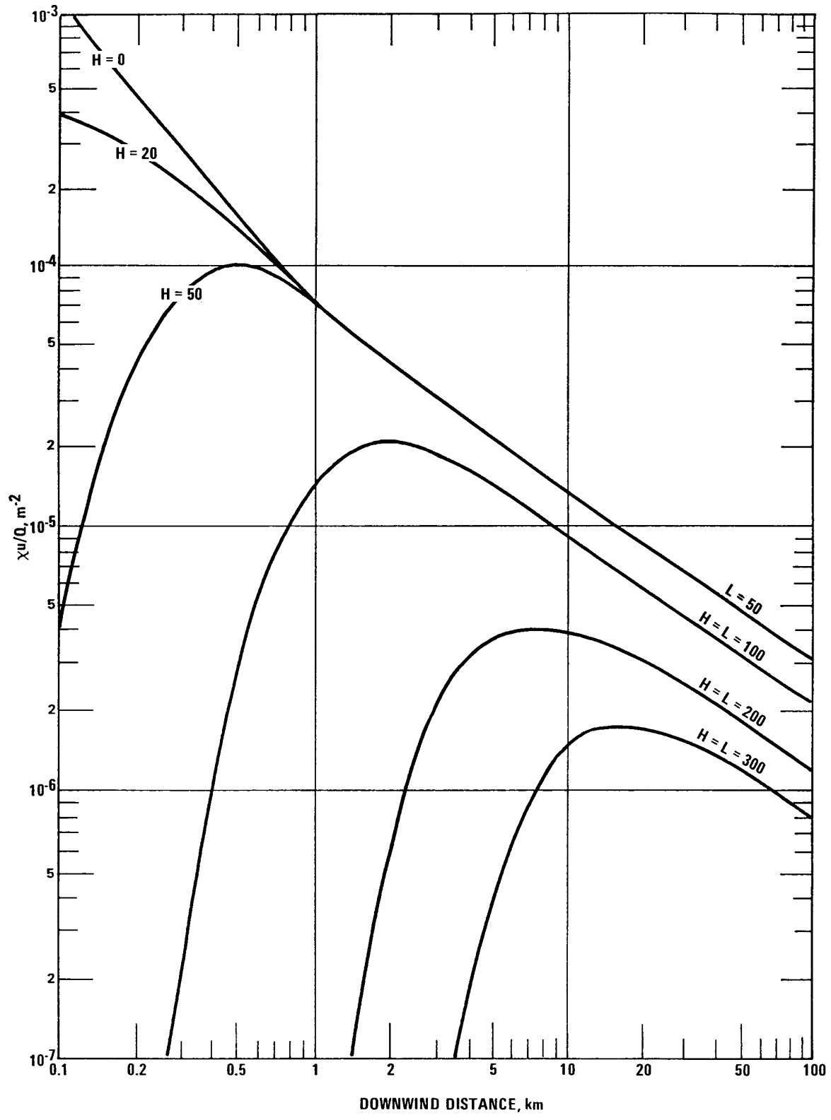
Figure 4-1 3.^^ ^Doc uen t Er- r o r^^ ^^ Doc- uen t Er- r o r^^ ^^ Sta- bility class E, urban ter- rain; u /Q vs. dis- tance for vari- ous plume height ts (H), as- sumin g very re- stricti ve mix- ing heigh ts (L); L = 50m for H ≤ 50m; L = H for H > 50m.
