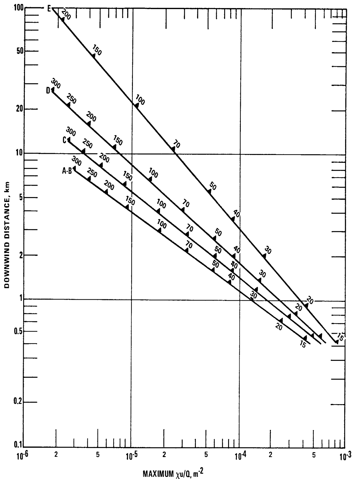
Figure 4-3. Document Error Document Error Document Error Downwind distance to maximum concentration and maximum \chi u/Q as a function of stability class for urban terrain. Plume heights (m) are indicated on the curves.
