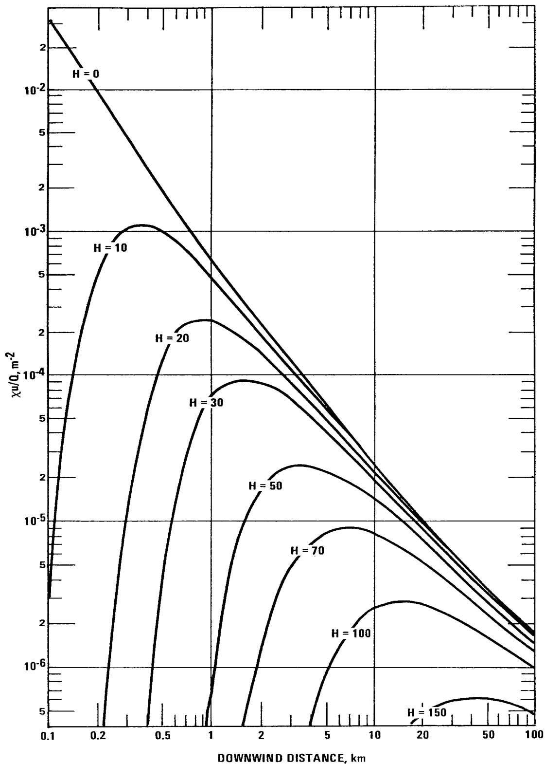
Figure 4-9. \chi u/Q vs. distance for various plume heights (H), assuming very restrictive mixing heights (L); L = 50m for H ≤ 50m; L = H for H > 50m.
