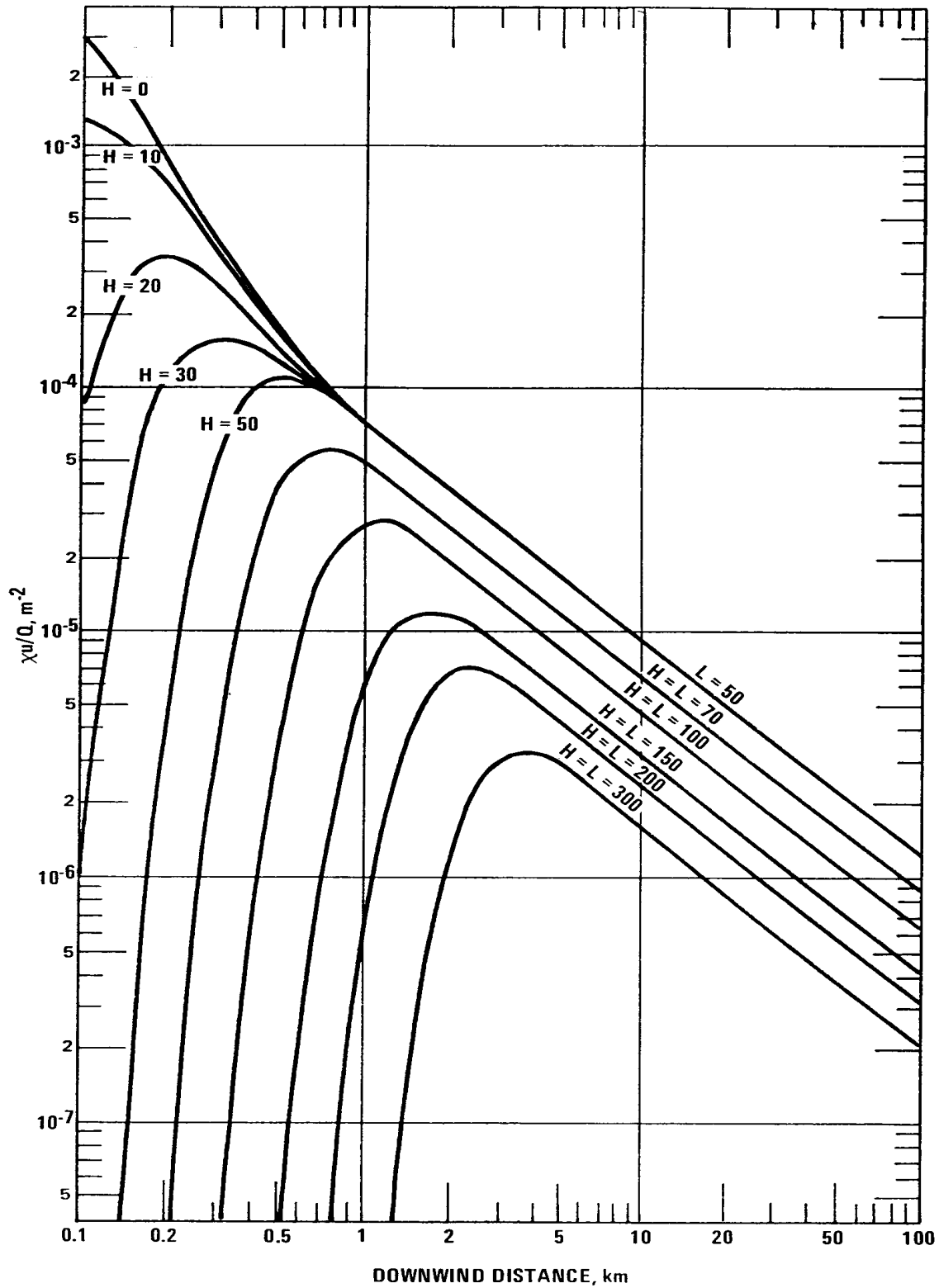
Figure 4-6. \chi u/Q vs. distance for various plume heights (H), assuming very restrictive mixing heights (L); L = 50m for H \leq 50 m; L = H for H > 50 m.
