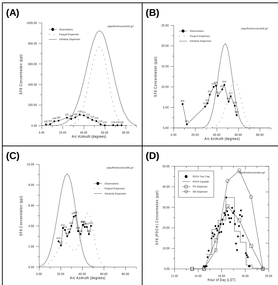
Figure 11. Six-hour average SF 6 concentration values observed and estimated for April 19, 1977, (A) 3.2-km arc, 1300-1900 MST; (B) 48-km arc, 1400-2000 MST; (C) 90-km arc, 1600-2200 MST. Azimuth is defined as viewed from the release position with 0 due North and 90 due East (see Figure 9). Receptor numbers are shown just above each observed concentration value. (D) Time history of observed PDCH and estimated SF 6 concentrations along the 48-km arc for April 19, 1977. Observed PDCH values were multiplied by 3.16 for comparison with estimated SF 6 values (volume of SF 6 divided by volume of PDCH released equals 3.16).
