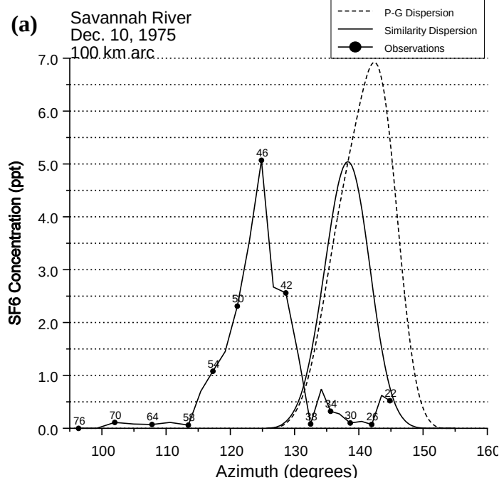
Figure 9. Simulated and observed seven-hour average concentration values along sampling arc for the Savannah River Laboratory December 10, 1975 tracer field experiment.
