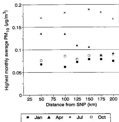
Figure 4. Highest monthly concentrations of (A) \text{SO}_2 , (B) \text{NO}_x , and (C) \text{PM}_{10} ( \mu\text{g}/\text{m}^3 ) from ring sources for January, April, July and October, 1988.
