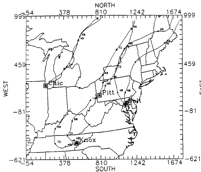
Figure 6. Trajectories at 10 m on the 54 km grid produced by CALMET (A) using the large radius of influence and observations only, and (B) using the large radius of influence and introducing the MM4 80 km winds in the Step 1 initial guess. CALMET results are shown with "o" and trajectories developed directly from MM4 54 km winds are shown with "x". The starting date was August 1, 1988 at 7 AM. The small numbers indicate hours after release.
