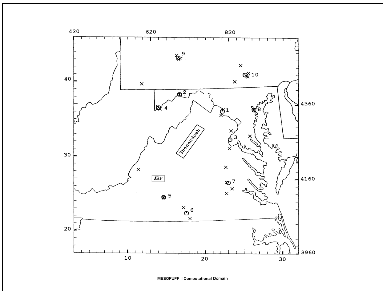
Figure 2. Display of the MESOPUFF II computational domain, showing positions of all PSD sources compiled for the demonstration assessment. Crosses represent all 27 original PSD sources, while circles denote the ten final aggregated sources used for the demonstration analyses. The source characteristics for the ten aggregate sources (numbered) are given in Table 2. One unit along left and bottom axes equals 20 km. Top and right axes are the UTM coordinates in km.
