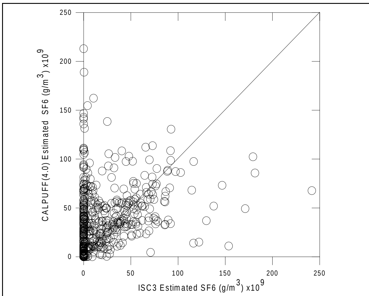
Figure 27. Scatter plot for Kincaid, comparing CALPUFF(4.0) and ISC3 simulation results for surface concentration values of SF 6 for Quality 2 and 3 data.
