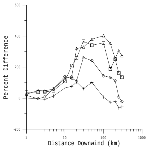
Figure 18. Percent differences (CALPUFF versus ISC3) as a function of downwind distance for the second-highest concentrations; (A) 1-hr, (B) 3-hr, (C) 24-hr, and (D) annual averages. Data are for Medford, Oregon.
