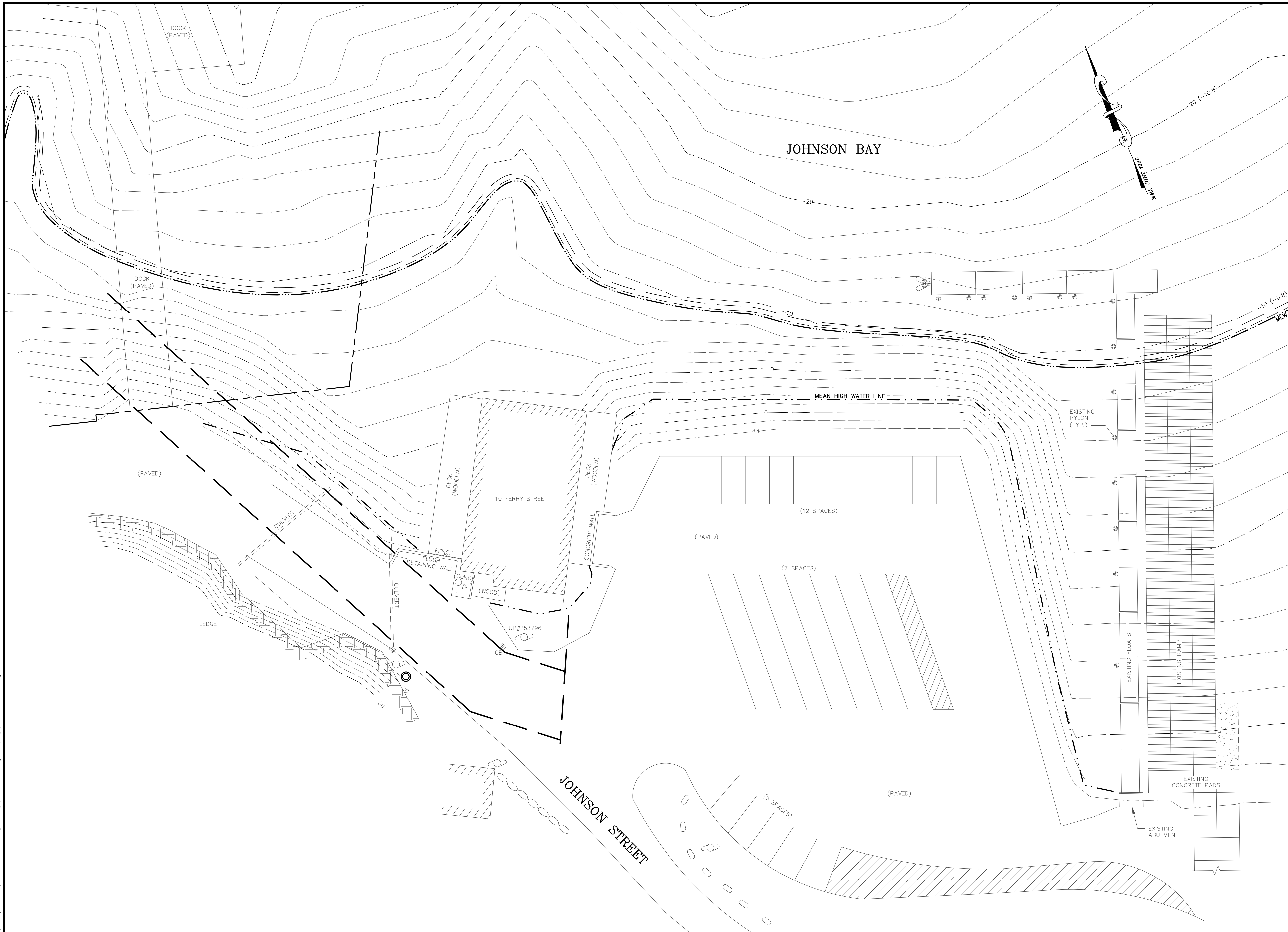
EXISTING CONDITIONS PLAN SCALE: 1" = 20'
