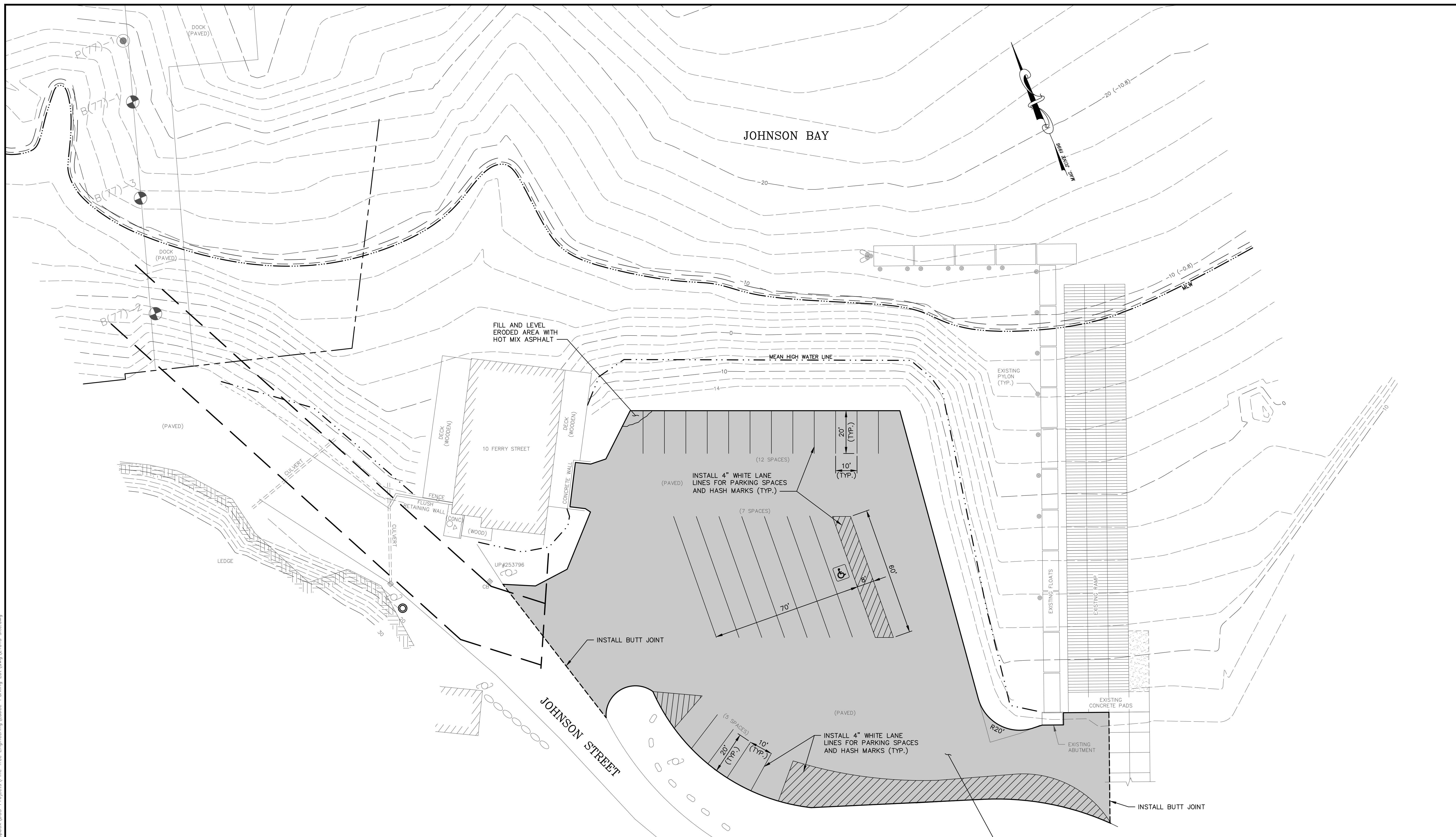
PROPOSED SITE PLAN SCALE: 1" = 20'
