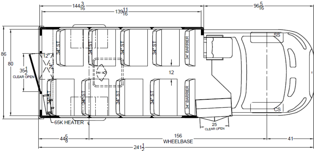
Floor Layout: Trans Star 16C/17A
