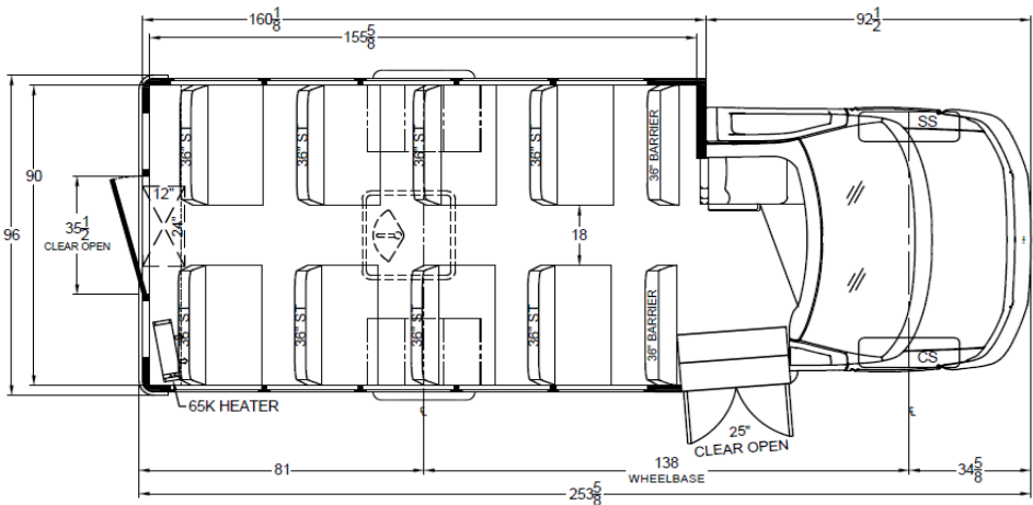
Floor Layout: SST 16C/17A
