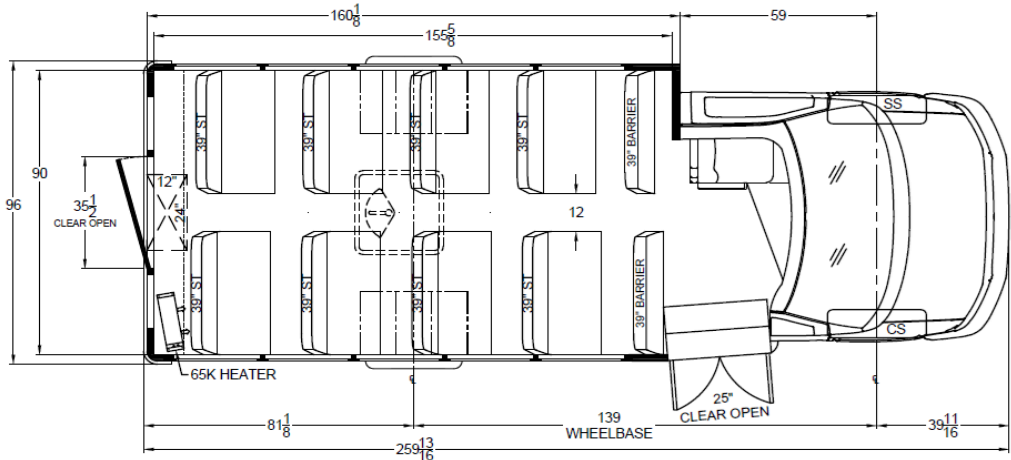
Floor Layout: SST 24C/17A
