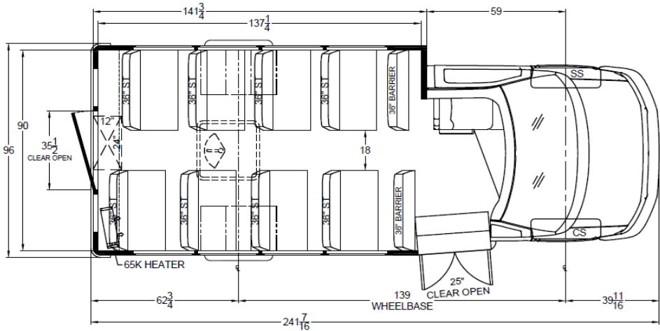
Floor Layout: SST 16C/17A
