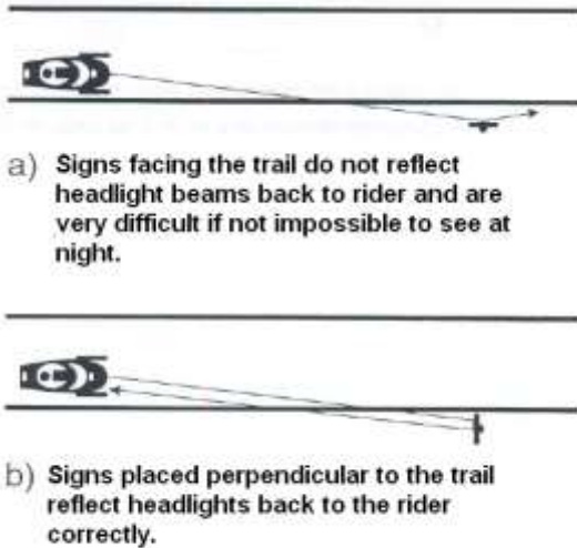
Figure 2 Sign Orientation, Plan View
