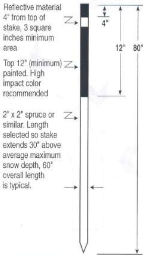
Figure 4 Typical Stake
