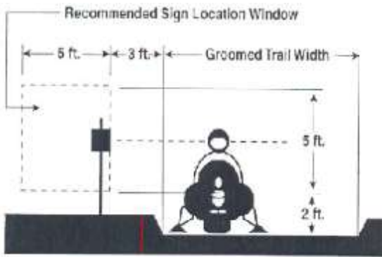
Figure 3 Recommended Sign Location Window
