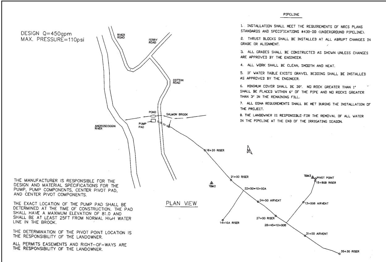
Pipe Plan 1
