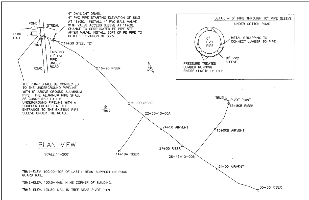
Pipe Plan 2
