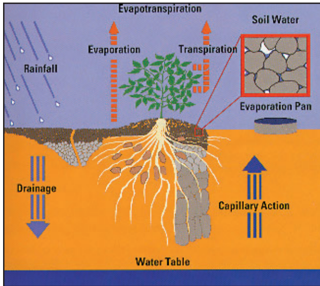
Evapotranspiration (Et) Cycle (Source: Best Management Practices: Irrigation Management . Ontario (Canada) Ministry of Agriculture, Food and Rural Affairs, 1995)
