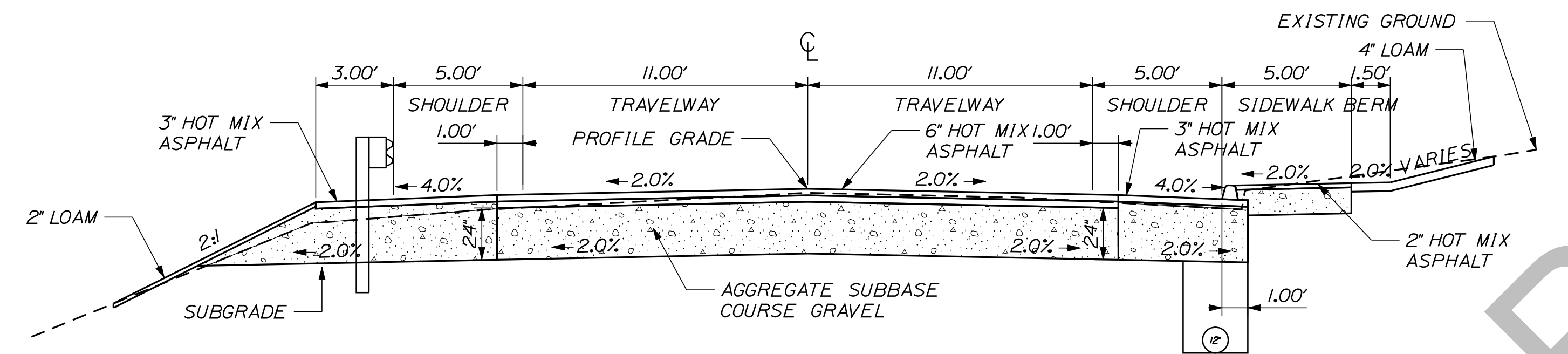
FULL CONSTRUCTION GUARDRAIL LEFT
