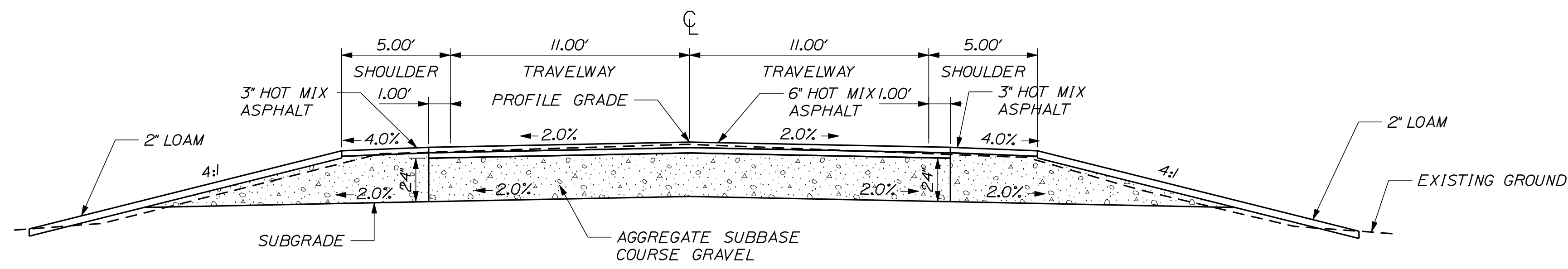
FULL CONSTRUCTION OPEN
