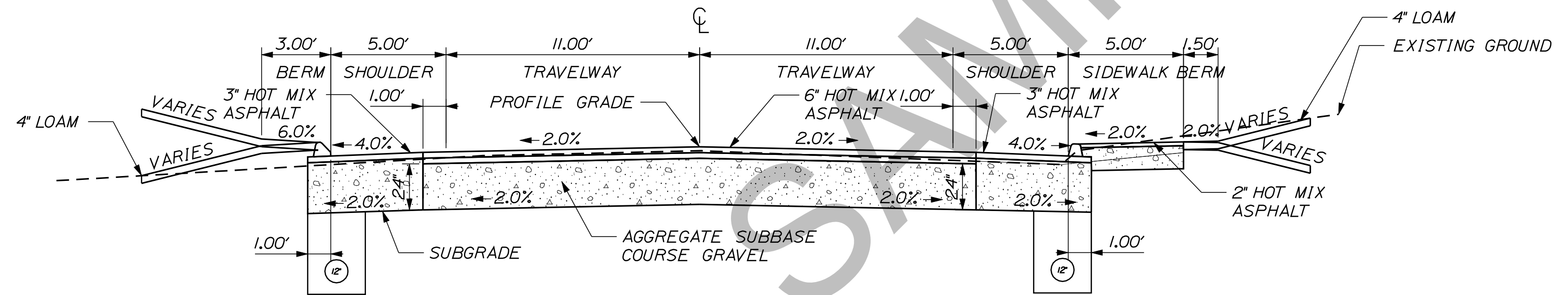
FULL CONSTRUCTION W/SIDEWALK
