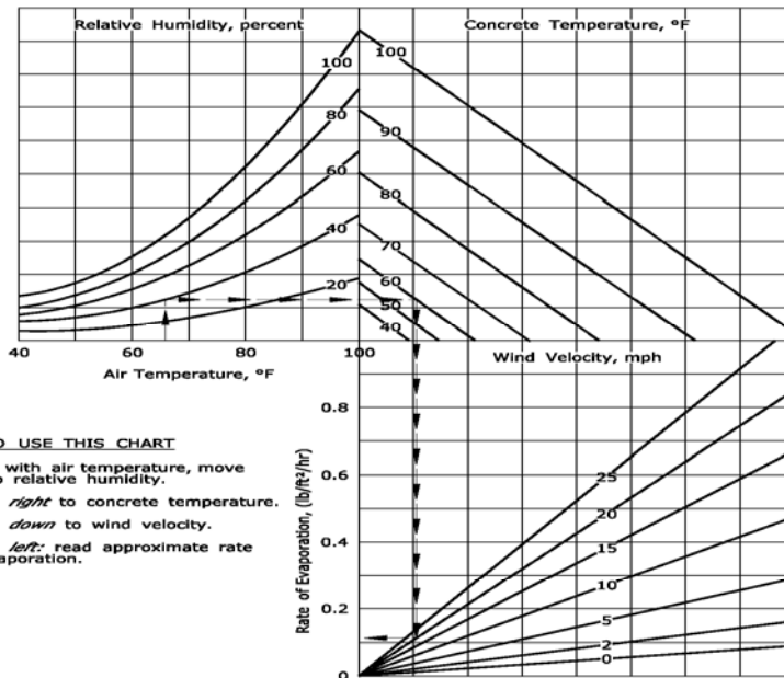
RATE OF EVAPORATION FROM CONCRETE SURFACE CHART
