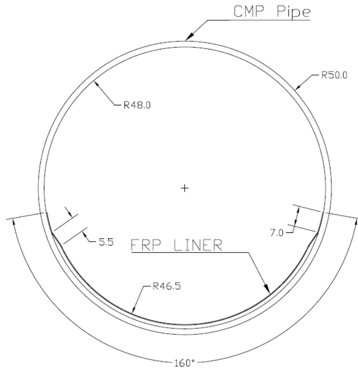
Figure 1 – Sample Liner Dimensions
