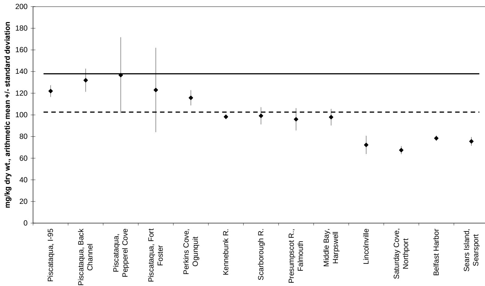
FIGURE 1.1.3.10.2: 2008 SWAT Blue Mussel Zinc Concentrations
