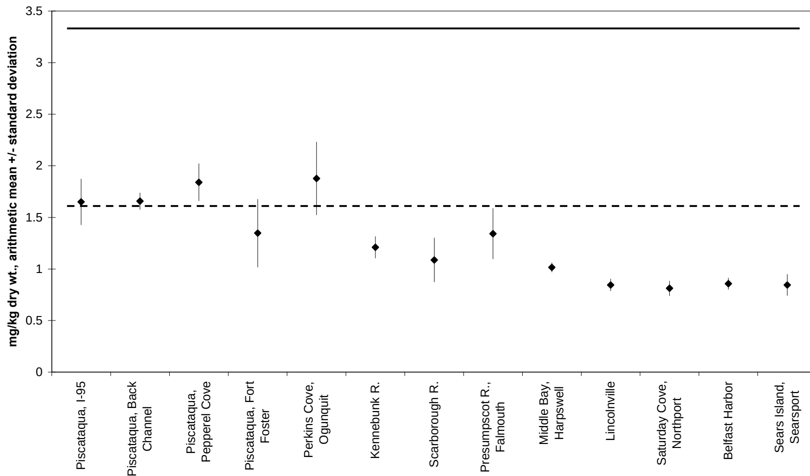
FIGURE 1.1.3.7.2: 2008 SWAT Blue Mussel Tissue Nickel Concentrations
