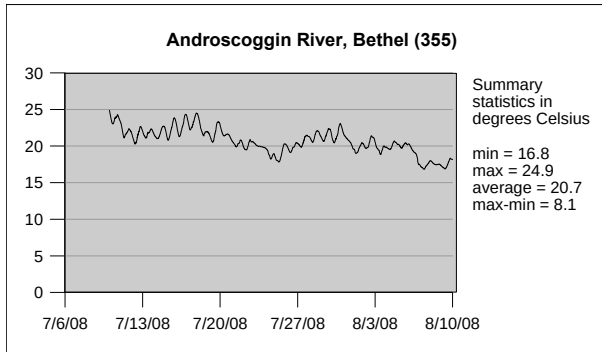
Figure 3.1.1 – 2008 In-Stream Temperature Data
