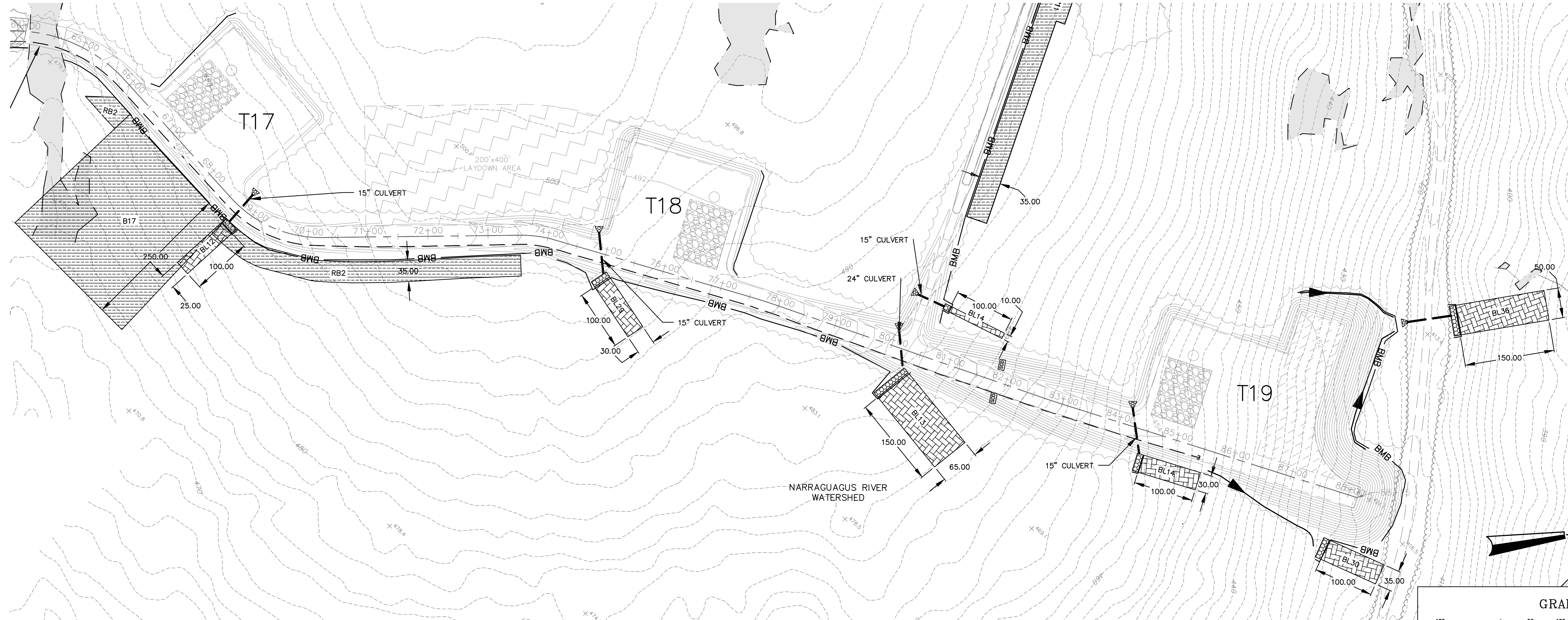
ALIGNMENT "NORTH STRING" - CRANE PATH (63+00 TO END CRANE PATH)
