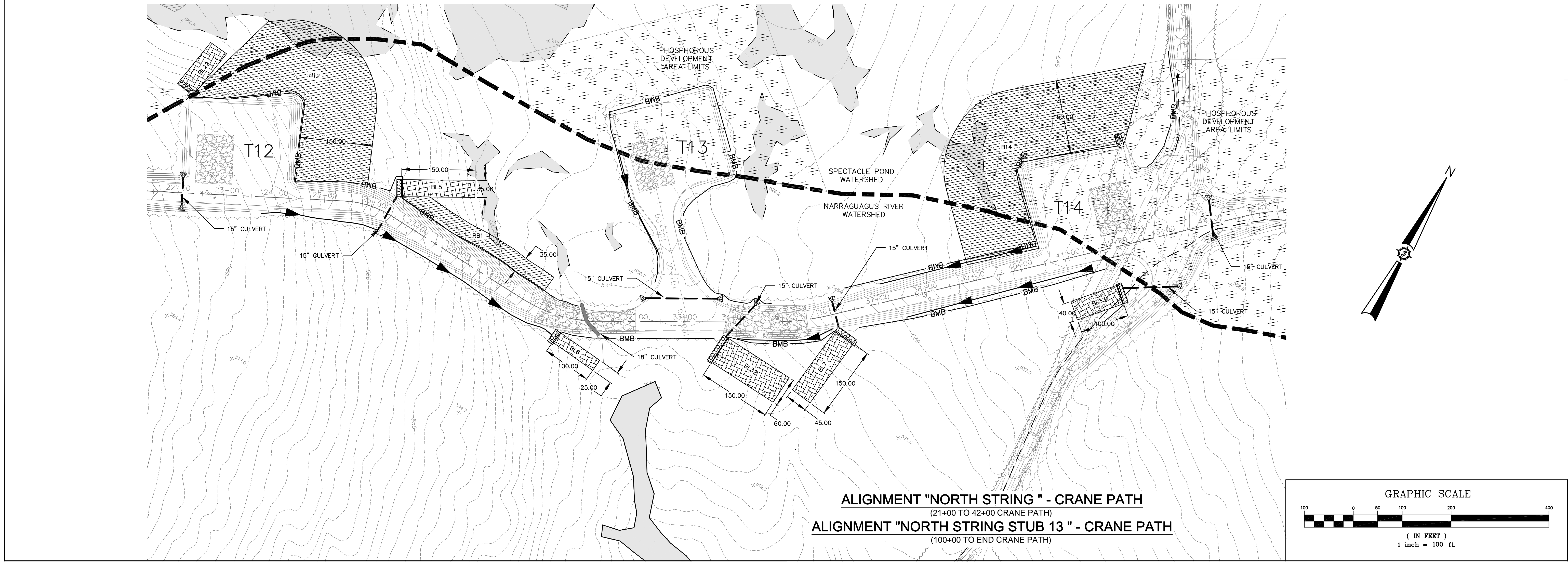
ALIGNMENT "NORTH STRING" - CRANE PATH (0+00 TO 21+00 CRANE PATH)
