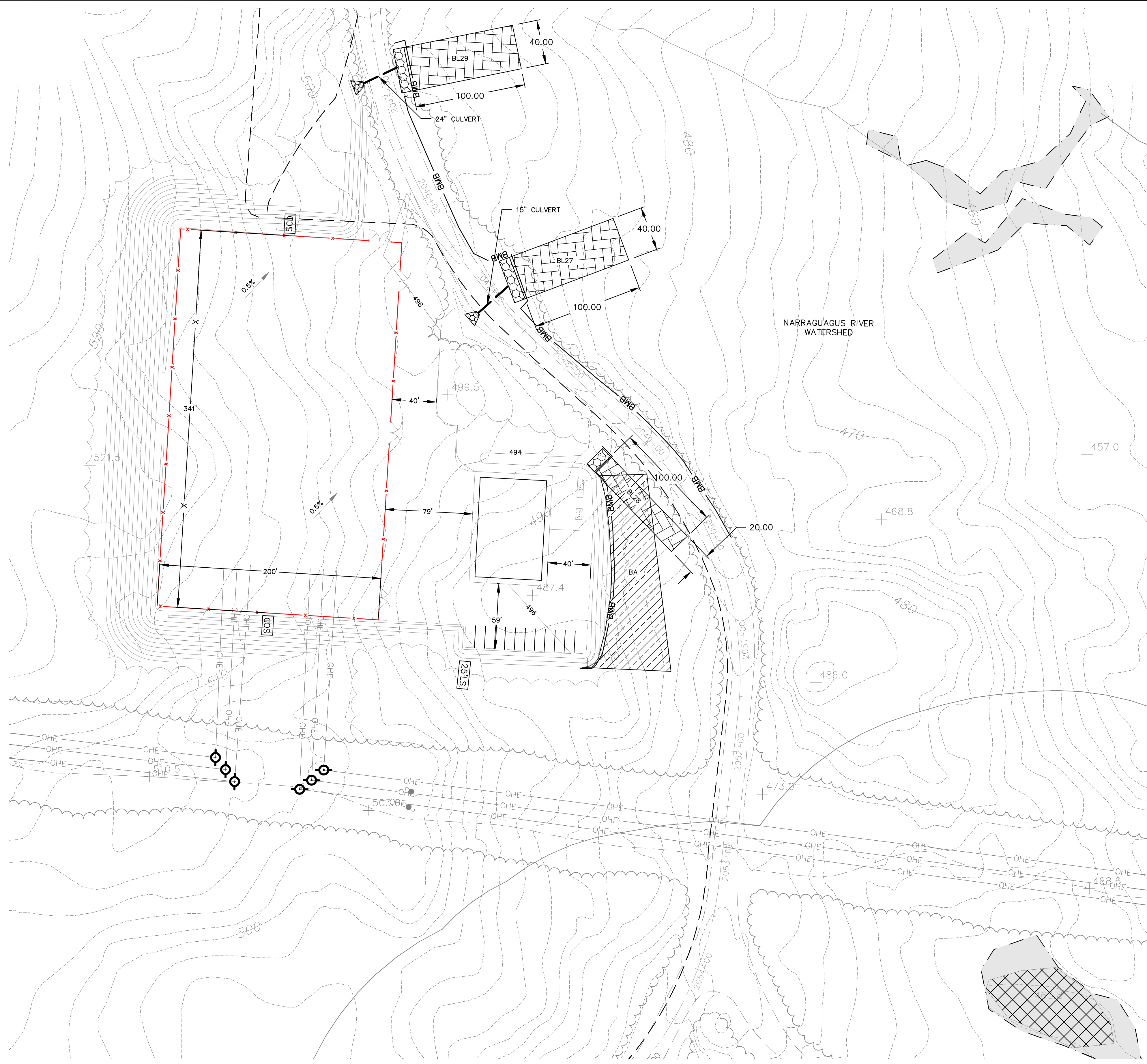
SUB STATION AND O&M BUILDING
