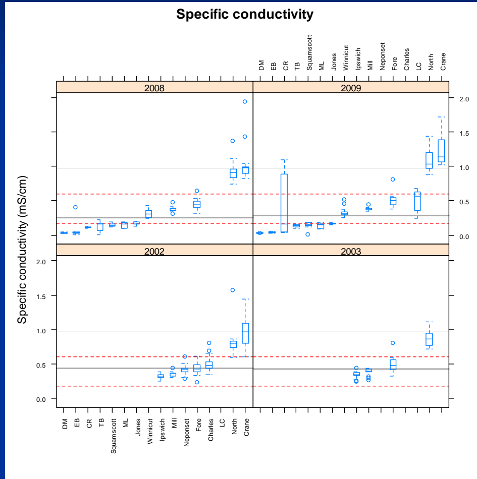
Boxplots of distribution of specific conductivity. Grayline is median for year. Red dashed lines are 25th and 75th quantiles for all years and rivers combined.
