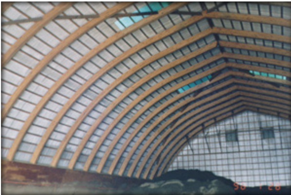
Interior of arch structure. Note "boxed in " and protected arch connections at top of concrete wall.
